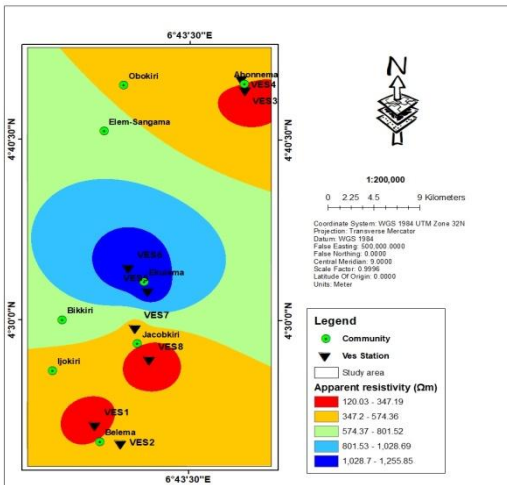
Fig.15: Apparent Resistivity map of study area
