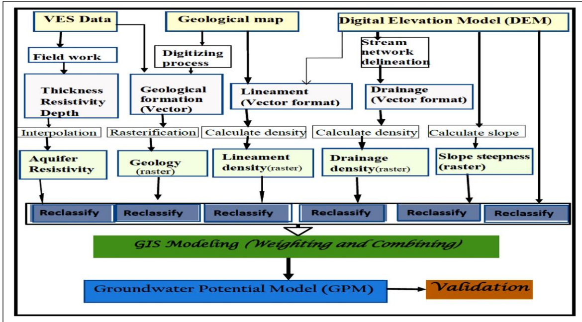
Fig. 3: Workflow of Groundwater Potential Model of Study Area [6]
