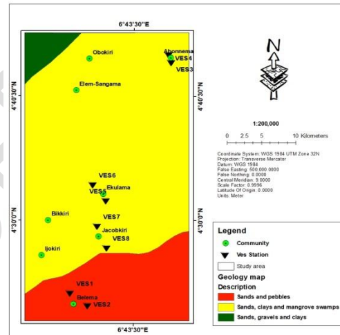
Fig.16: Geology map of study area
