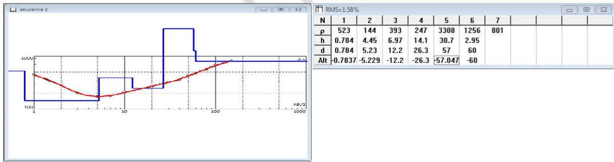
Fig. 7: VES a. Curve type of Ekulama2 b. Model of Ekulama2
