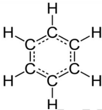
Figure 3.: Structure of Benzene Source: Bahadar et al. ,(2014)
