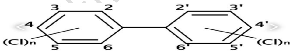
Figure 5: Structure of Polychlorinated Biphenyls Source: Longnecker et al. , (2021)
