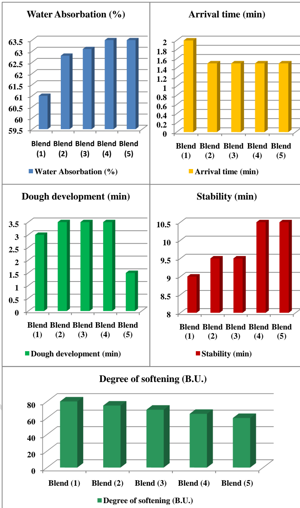
Fig.1. Rheological characteristics for different treatments balady bread with farenograph.
