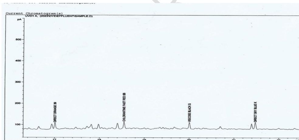
Fig. 3: Chromatogram of the Textile Effluent obtained through HPLC
