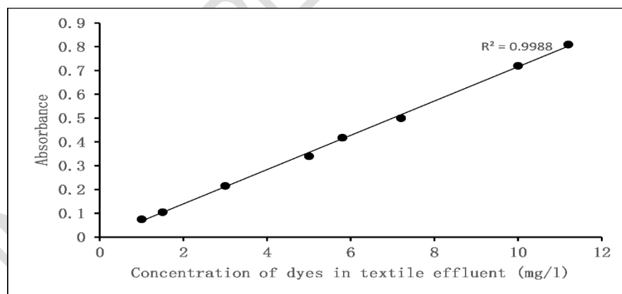
Fig. 4: Calibration curve of the dyes concentration (mg/l) at \lambda_{\max} = 510 nm)
