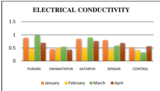
Figure 2: Effect of Jallaxmi Cement Factory, on Soil EC at study sites in different Months.
