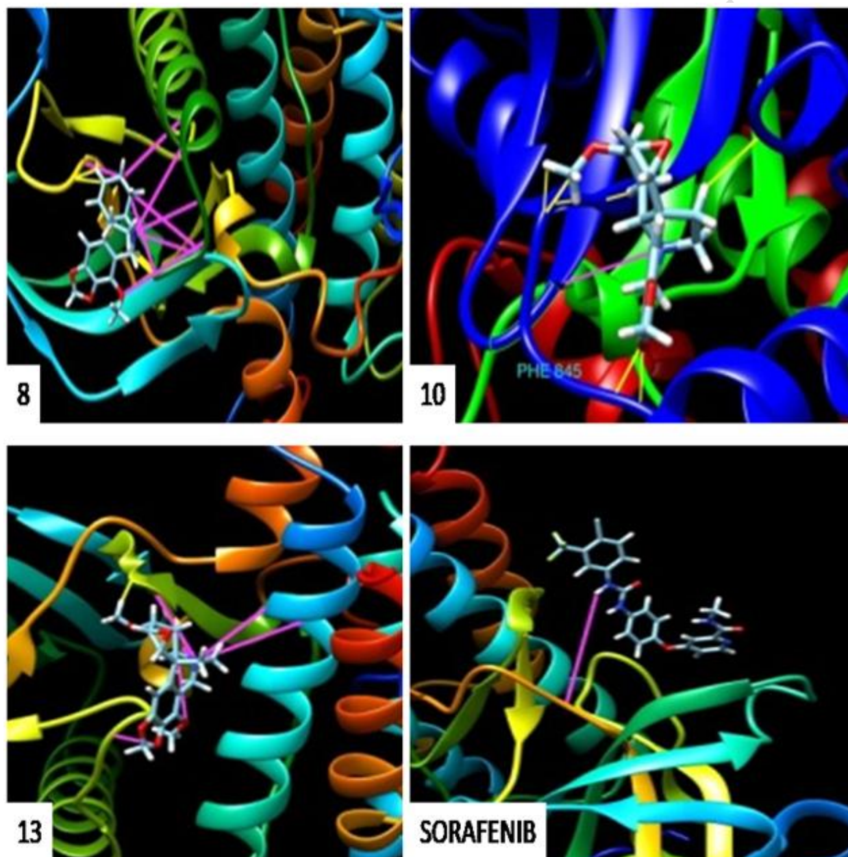
Figure 3: Docking poses of selected crinine alkaloids against 3VHE
