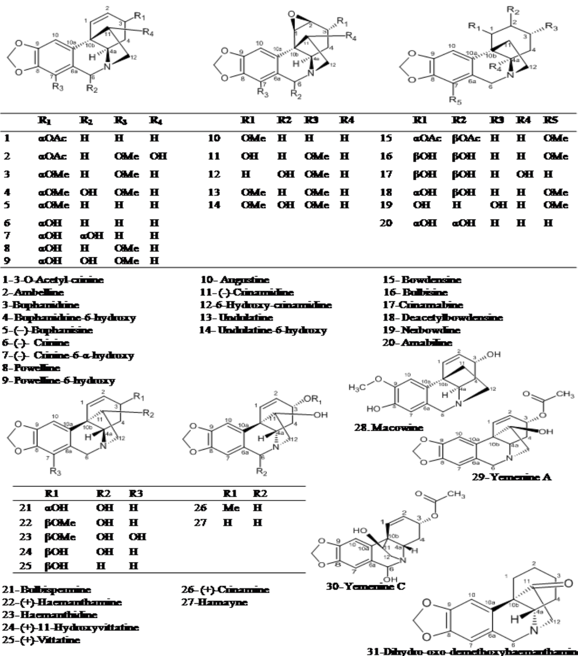
Figure 1: Structures of Crinine alkaloids under investigation
