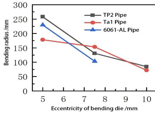
Fig. 10.comparison of bending radius of different tubes
