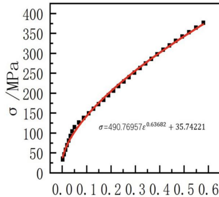
Fig. 3. \sigma - \varepsilon fitting curve
