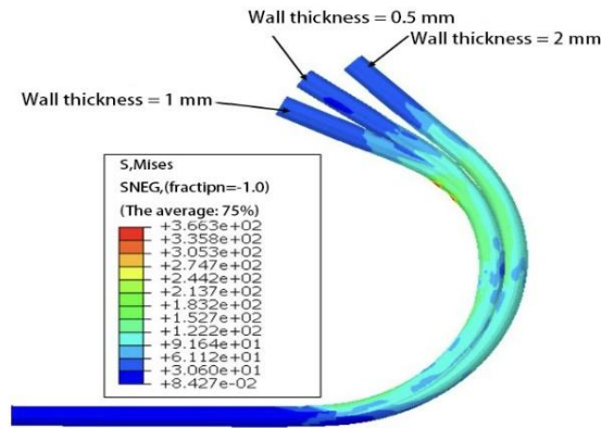
Fig. 9.bending deformation of tube under different wall thickness
