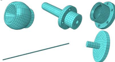
Fig. 5. Mesh division of each component
