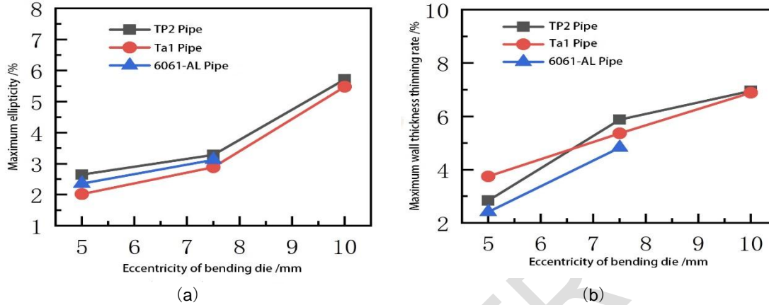
Fig. 11.variation of maximum change rate of different tubes with eccentricity
