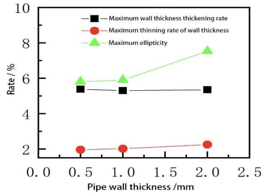
Fig. 8.relationship between tube change rate and wall thickness
