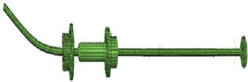
Fig.3. Finite element model of pipe bending
