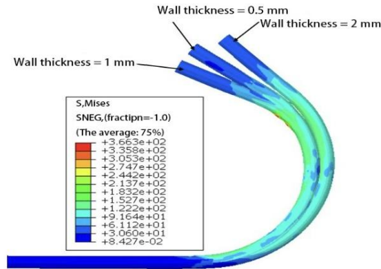
Fig. 8. bending deformation of tube under different wall thickness
