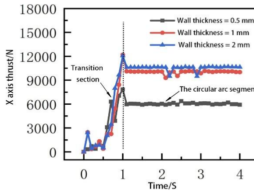
Fig. 6. variation of x-axis thrust of tube under different wall thickness
