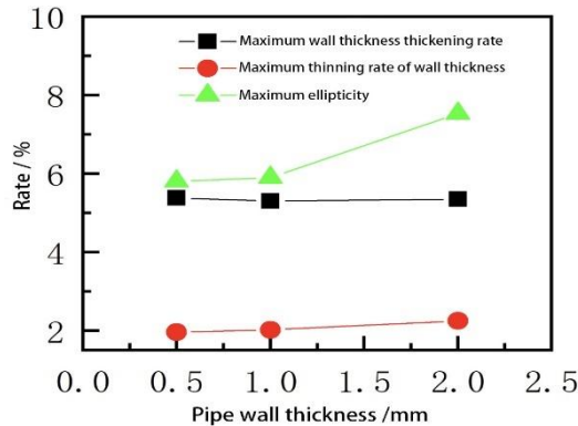
Fig. 7. relationship between tube change rate and wall thickness
