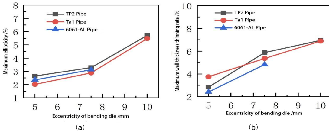
Fig. 10. variation of maximum change rate of different tubes with eccentricity
