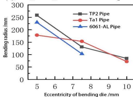
Fig. 9. comparison of bending radius of different tubes
