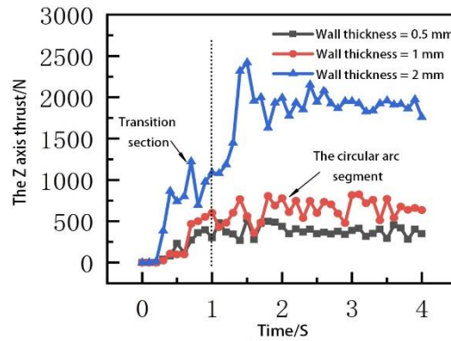
Fig. 5. variation of z-axis thrust of tube under different wall thickness
