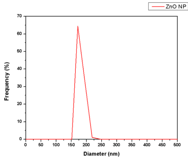
Figure 1. Particle size analysis of biosynthesized zinc oxide nanoparticles
