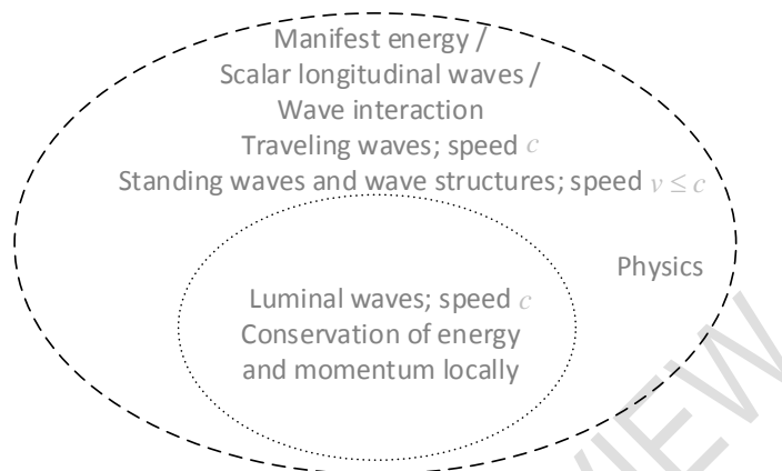
Fig. 2: Venn diagram of luminal and scalar longitudinal waves showing that luminal waves represent a less fundamental level.
