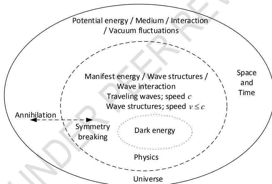
Fig. 1: A Venn diagram of “the model of physics” as obtained from [4], [5], [19]. Slashes indicate equivalences.
