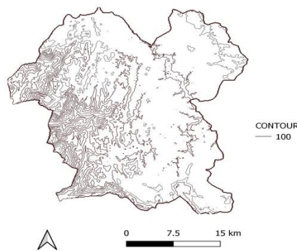
Fig. 6. Contour Map
