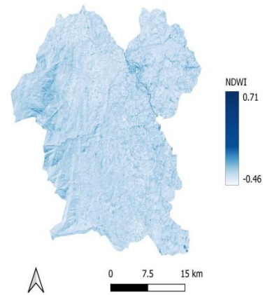
Fig.4. NDWI Map
