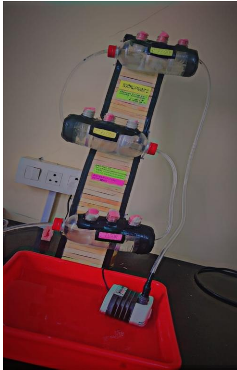
Fig 2: NFT system Hydroponics Model
