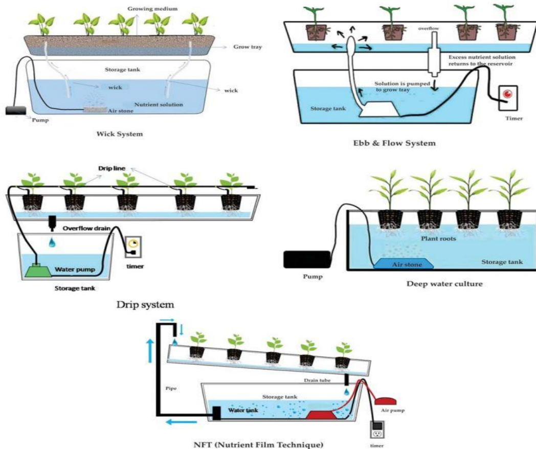
Fig. 1. Diagram of various structures of hydroponic system
