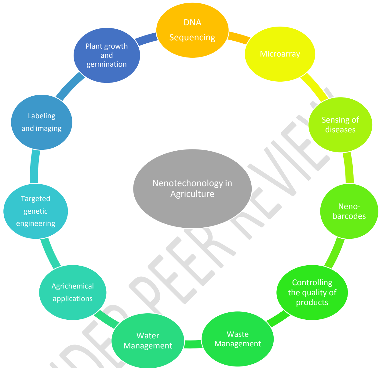
Fig. 1 Google Source of the Nanotechnology applications in agriculture.
