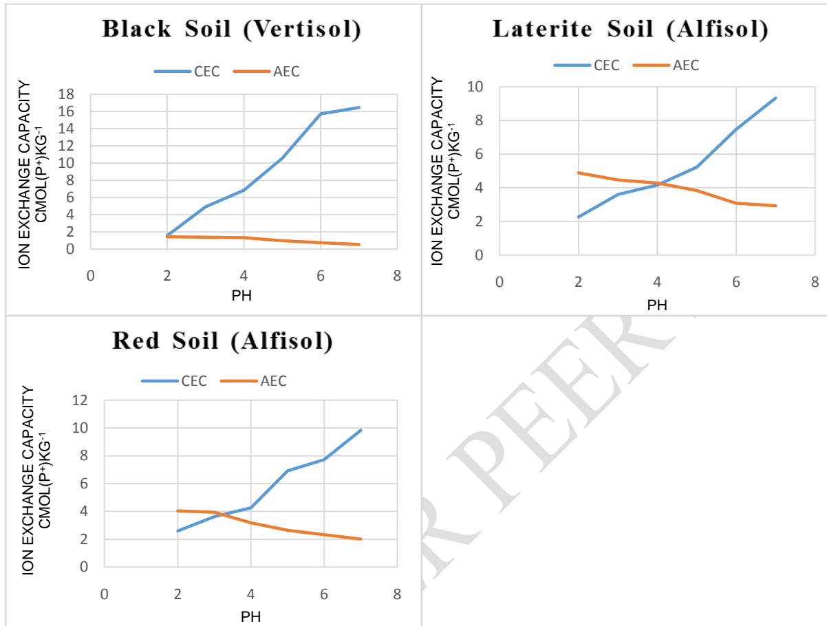
Figure 2. Point of zero net charge (PZNC) of the soil samples
