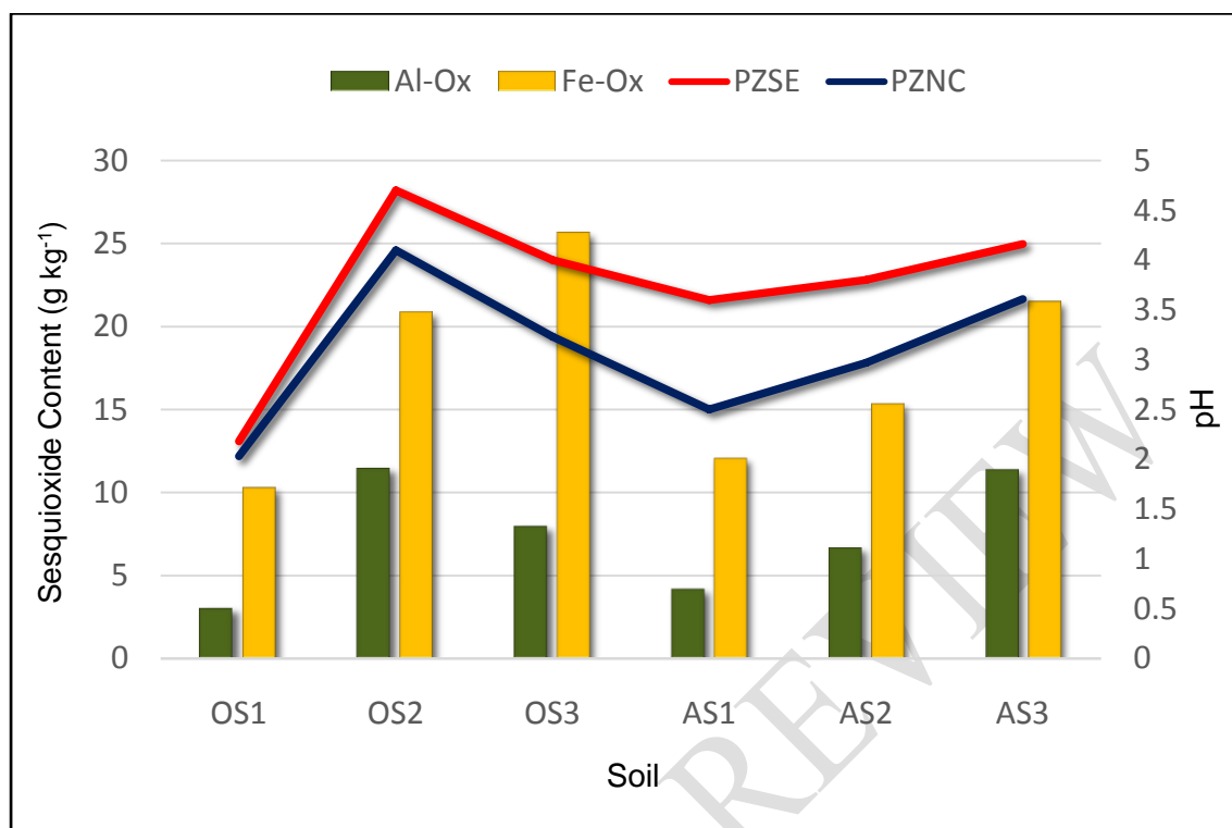
Figure 3. Relation between sesquioxides content in soil and PZC components
