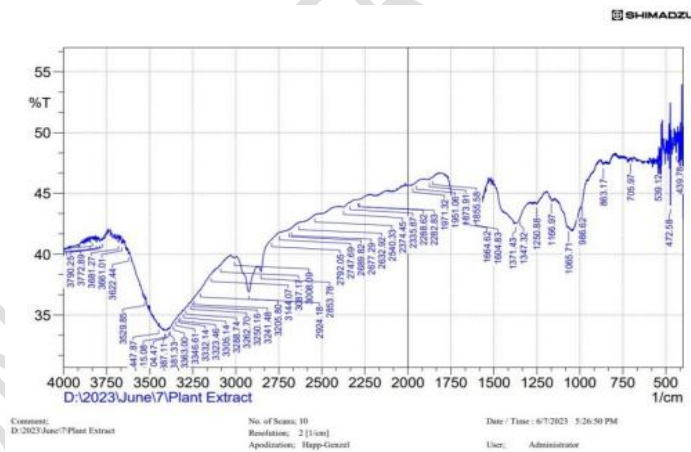
Fig 6: FT-IR Spectrum of Millingtonia hortensis leaves extract
