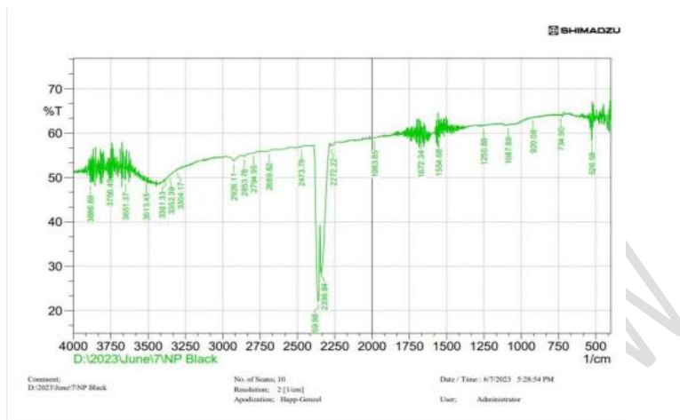
Fig 5: FT-IR Spectrum of synthesized silver nanoparticles using leaves extract of Millingtonia hortensis
