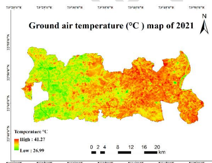
Fig. 14: Ground air temperature map of the study area in 2021
