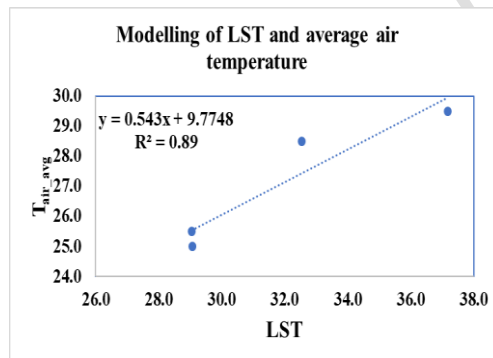
Fig. 8: Correlation of LST with average air temperature
