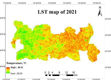
Fig.10: Land Surface Temperature (LST) map of 14 March 2021
