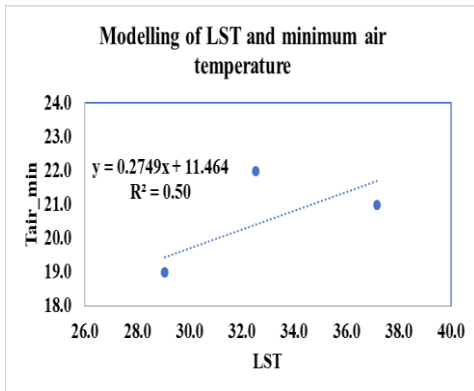
Fig. 6: Correlation of LST with minimum air temperature
