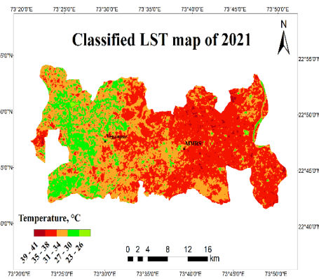
Fig.12: Different Land Surface Temperature (LST) classes map of 14 th March 2021
