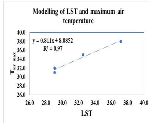
Fig. 7: Correlation of LST with maximum air temperature
