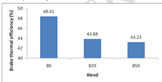
Fig 6: Effect of various blends on brake thermal efficiency
