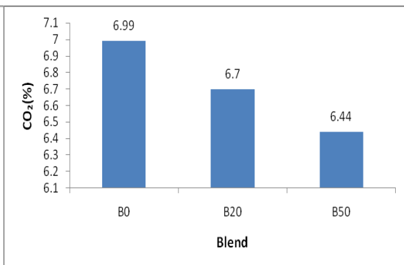
Fig 11: Effect of various blends on CO 2 emission
