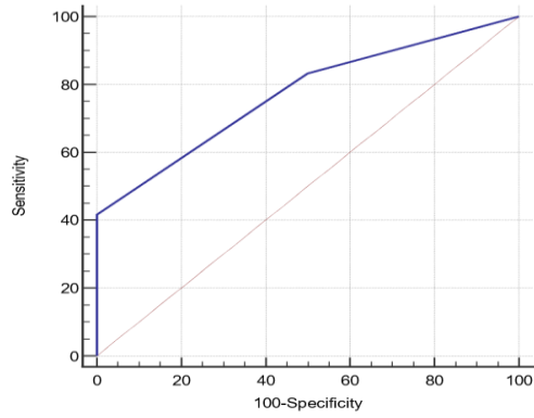
Figure 1: ROC curve of (A) NRI, (B) PNI, (C) CONUT scores in prediction of complications
