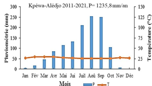
Figure 2 : Umbrothermal curve
