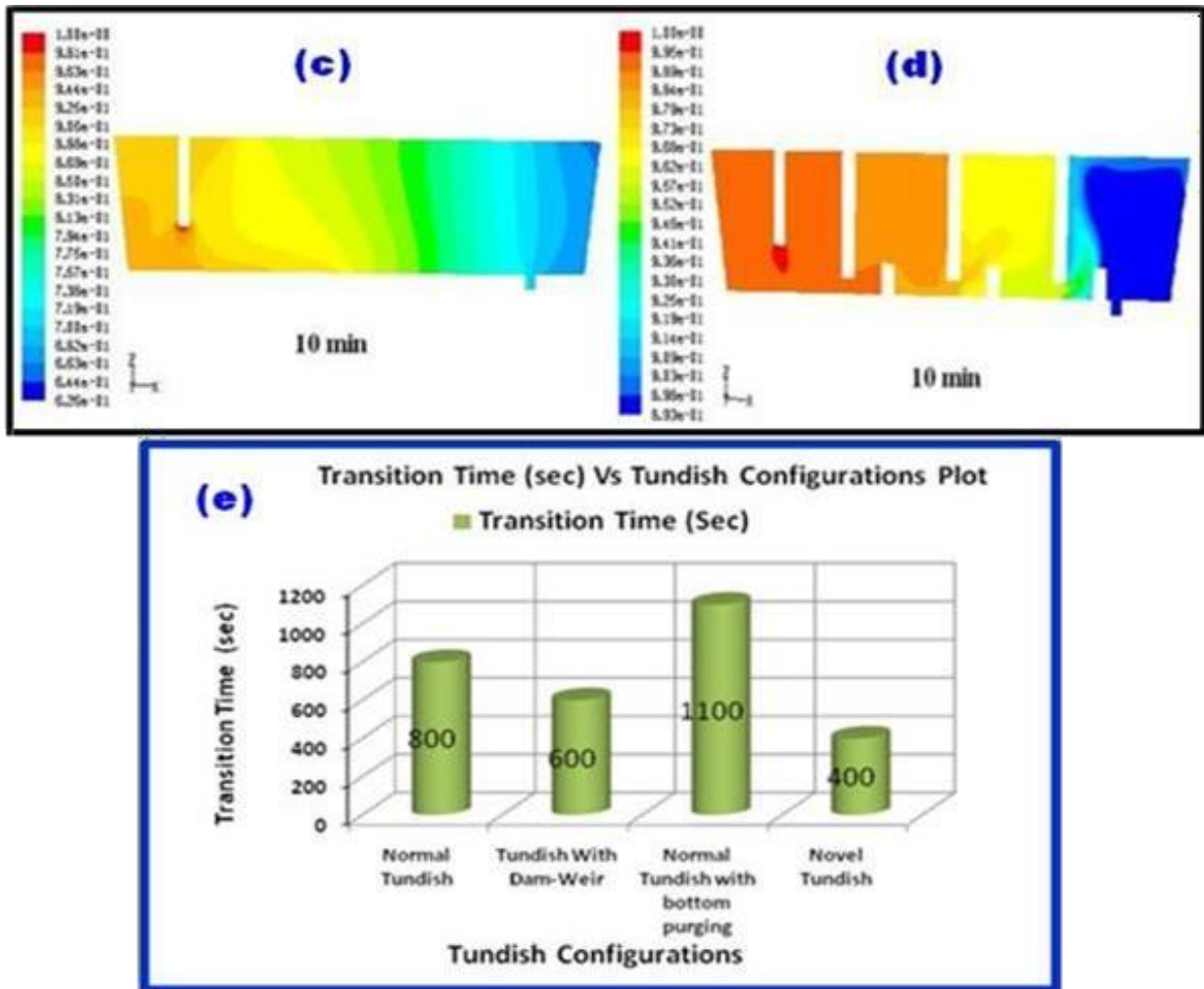
Figure 2 (a) Schematic of Multi Reactor Tundish with Argon Purging, (b) Schematic thereactor arrangement, (c)Grade mixing contour for Normal tundish without flow controlrefractory,(d)GrademixingcontourforNovelMultiReactortundish with argonpurging, (e) Transition time plot of different tundish configurations along with Novel Multi ReactorTundishwithargonpurging[13].
