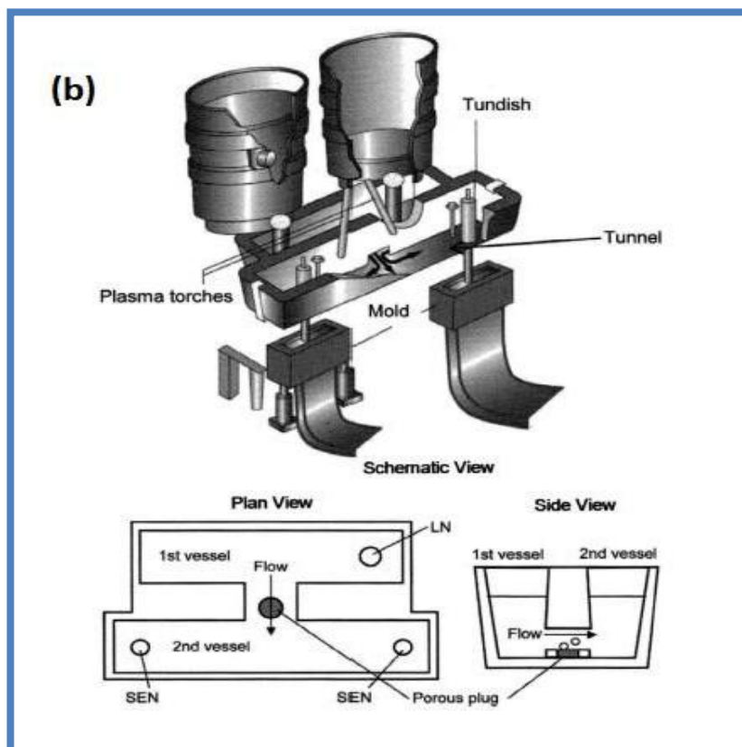
Figure 5(a) Centrifugal Flow Tundish (b) H-Shaped Tundish [28]
