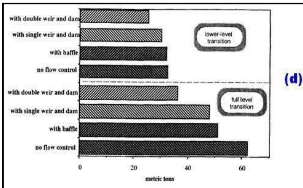
Figure 1 (a) Grade Transition in 45 ton Twin Strand Slab caster (b) Variation of mixed grade along slab length and width (c) Double weir-dam arrangement for reducing transitions (d) Amount of reduction in transitions at various tundish operations [3-4].
