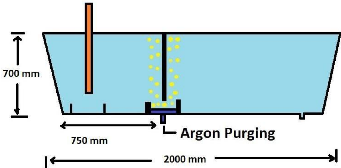
Figure7.Model NovelTundishGeometrywithDimensions
