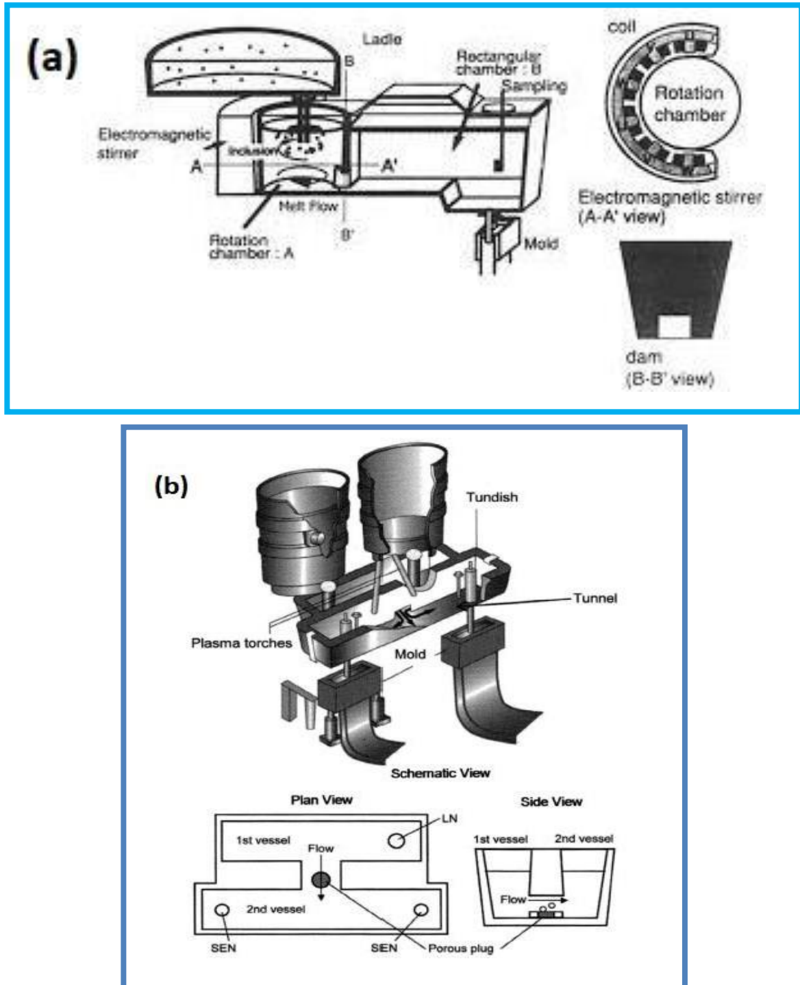
Figure 5 (a) Centrifugal Flow Tundish (b) H- Shaped Tundish [28]
