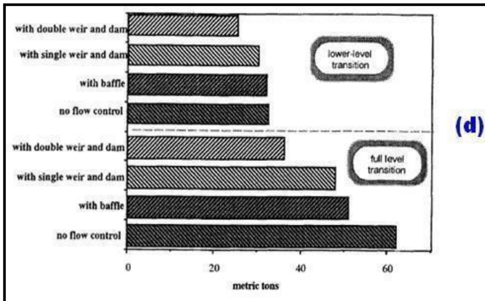
Figure 1 (a) Grade Transition in 45 ton Twin Strand Slab caster (b) Variation of mixed grade along slab length and width (c) Double weir-dam arrangement for reducing transition slab (d) Amount of reduction transition slab at various tundish operations [3-4].
