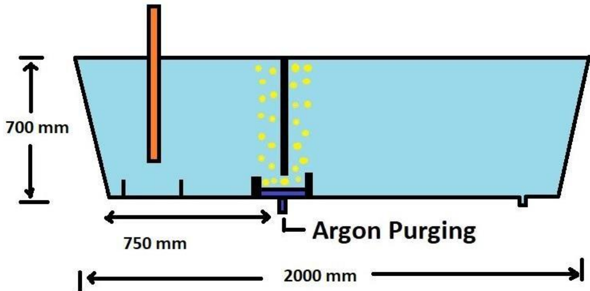
Figure 7. Model Novel Tundish Geometry with Dimensions
