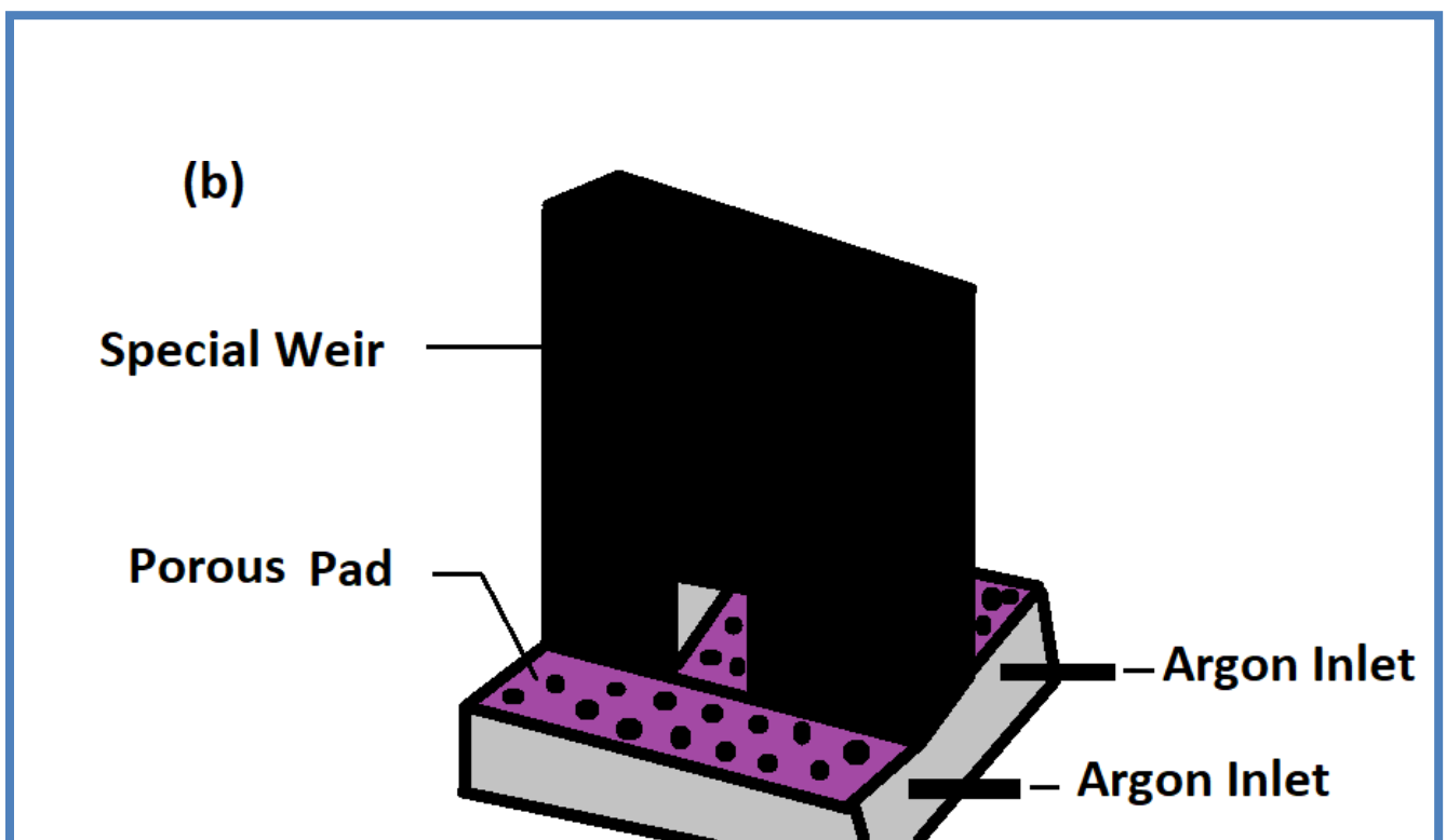
Figure 6 (a) Schematic of Novel Filter Tundish (b) Schematic of the Special weir with Argon Purging Pad.
