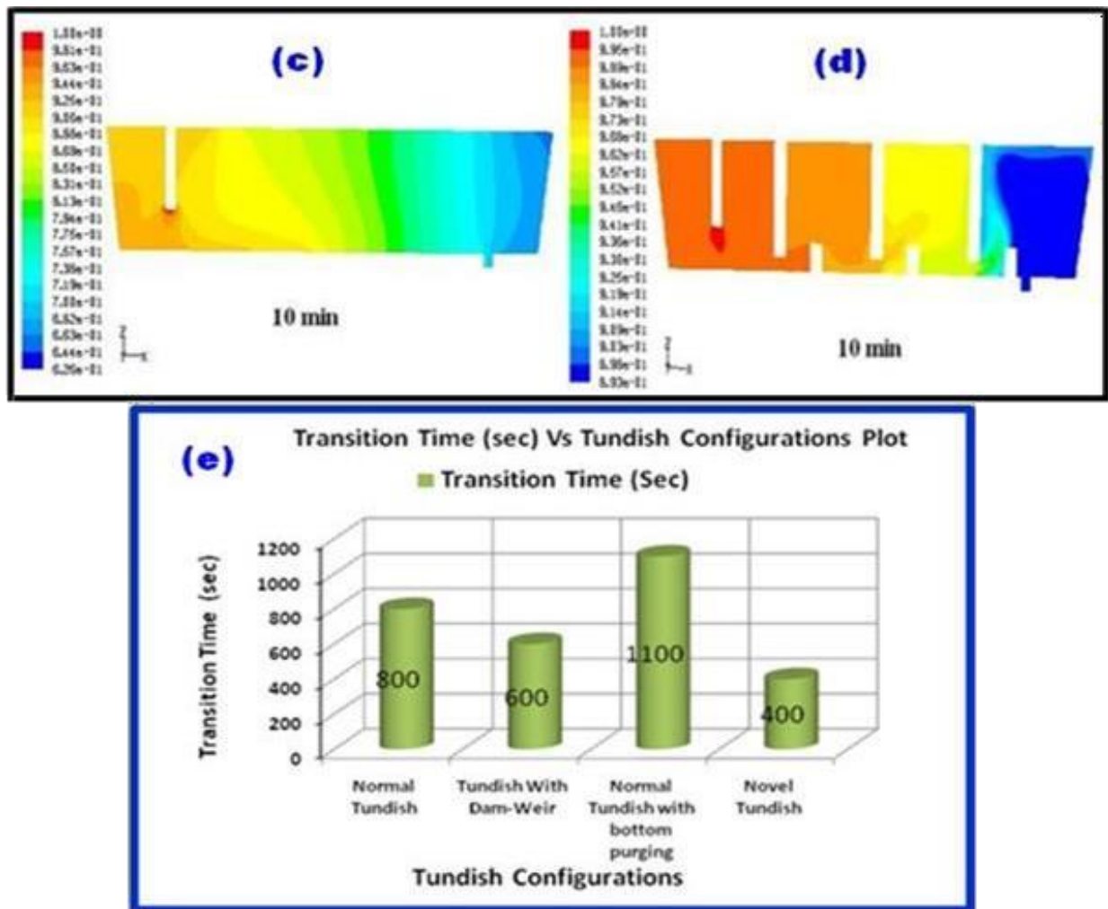
Figure 2 (a) Schematic of Multi Reactor Tundish with Argon Purging, (b) Schematic the reactor arrangement, (c)Grade mixing contour for Normal tundish without flow control refractory, (d) Grade mixing contour for Novel Multi Reactor tundish with argon purging, (e) Transition time plot of different tundish configurations along with Novel Multi Reactor Tundish with argon purging [13].
