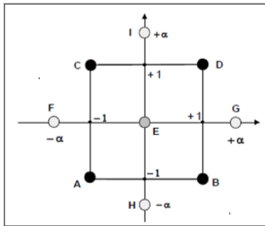
Figure 1: Graphic interpretation of experimental points of a central composite design with two factors [30].
