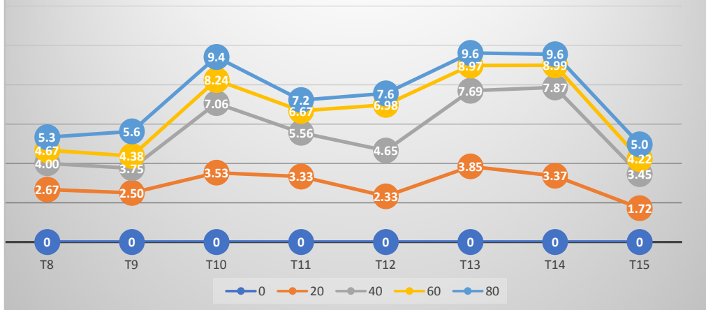
Fig 1.5: Percent increase in total-Zn from prepared enriched vermicompost when incubated with biofertilizers under different treatments
