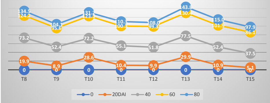
Fig 1.2a: Percent increase in available-P from prepared enriched vermicompost when incubated with biofertilizers under different treatments
