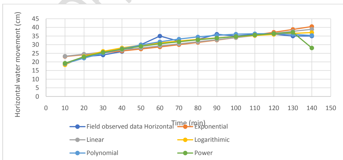
Graph 4: Comparison of observed wetting pattern in Horizontal path with statistical models.
