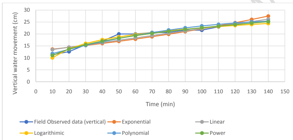
Graph 3: Comparison of observed wetting pattern in vertical path with statistical models.
