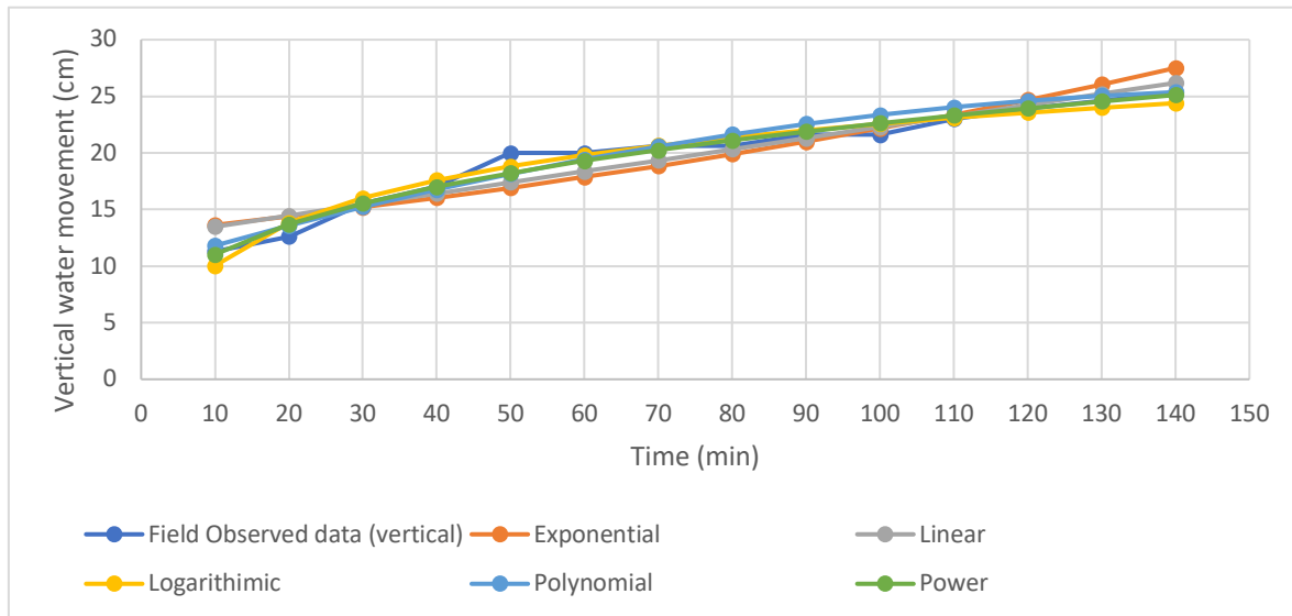
Graph Fig. 3 Comparison of observed wetting pattern in vertical path with statistical models
