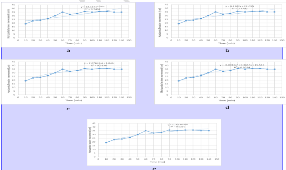
Graph Fig. 2 for Observed Horizontal water movement a (Exponential Model), b (Linear Model), c (Logarithmic Model), d (Polynomial model), e (Power Model).
