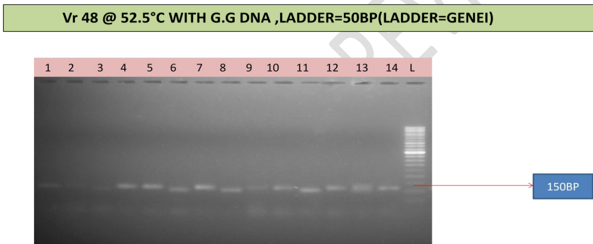
Figure 2: Image of DNA Banding pattern generated by Agarose gel electrophoresis of SSR VR 48 marker for 14 green gram genotypes
