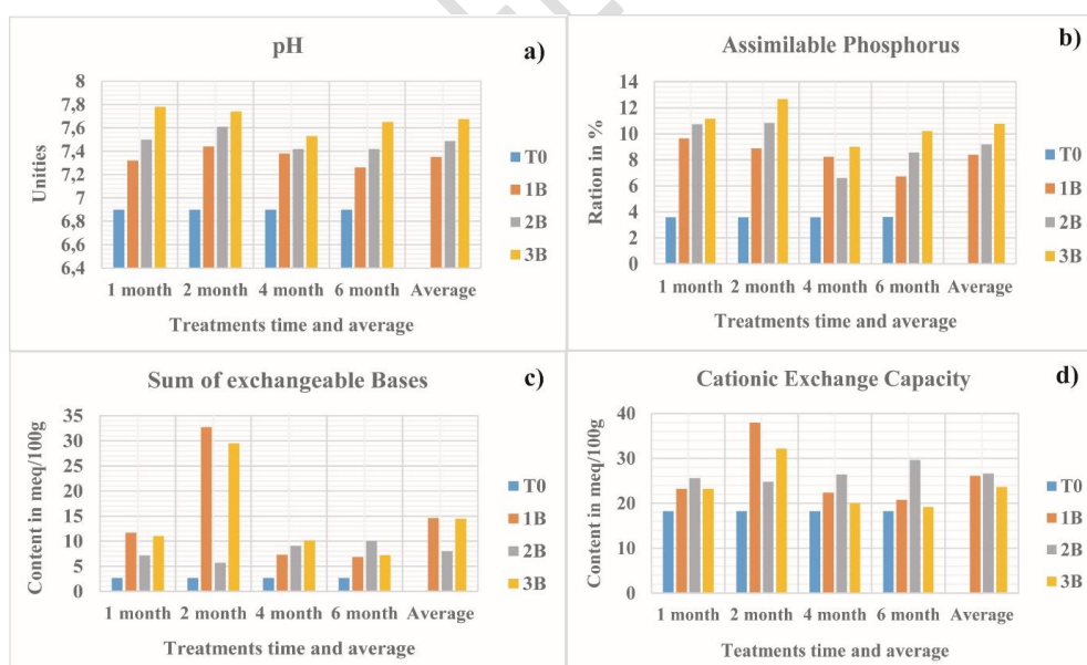
Fig. 3. Variation in pH (a), assimilable phosphorus (b), sum of exchangeable bases (c) and cation exchange capacity (d) diagrams.
