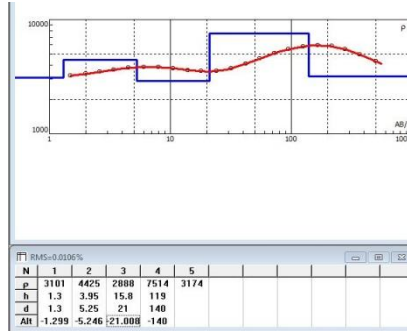
Figure 1: VES of Umuuanu
