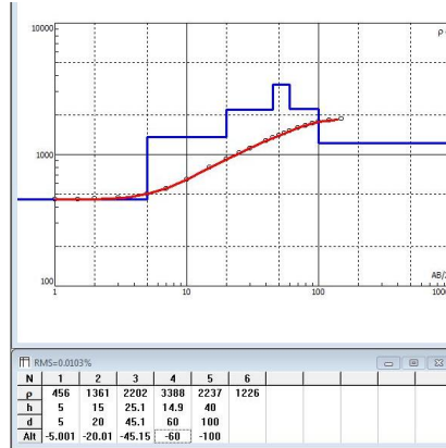
Figure 5: VES of Umudike
