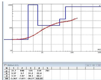
Figure 3: VES of Amaju
