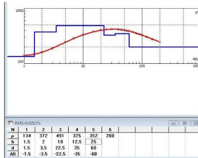
Figure 2: VES of Umuleke
