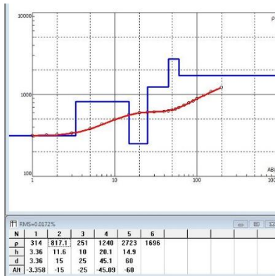
Figure 6: VES of Umuchoke
