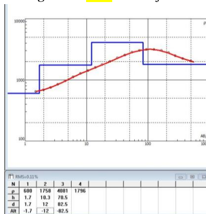
Figure 4: VES of Umudurumba
