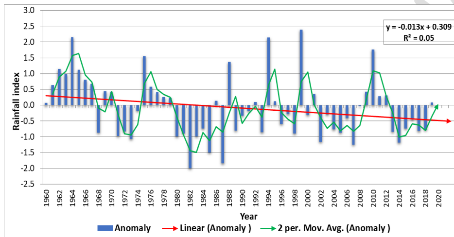
Figure 3.4. Interannual variability of rainfall for Segou (green line is moving average and red line is linear trend forecasting)
