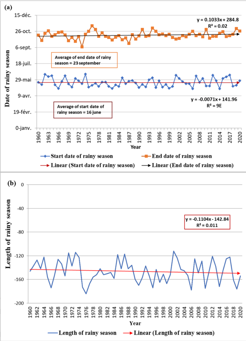
Figure 3.10. Trend of start and end of the rainy season (a), and the length trend of the rainy season (b) for Sikasso
