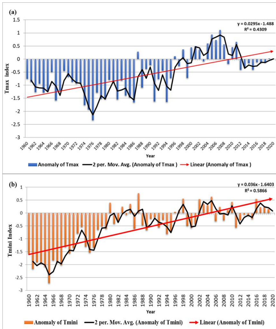
Figure 3.12. Anomaly trend of maximum (a) and minimum temperature (b) for Segou from 1960-2020 (red line a, b is linear trend and black line is moving average)
