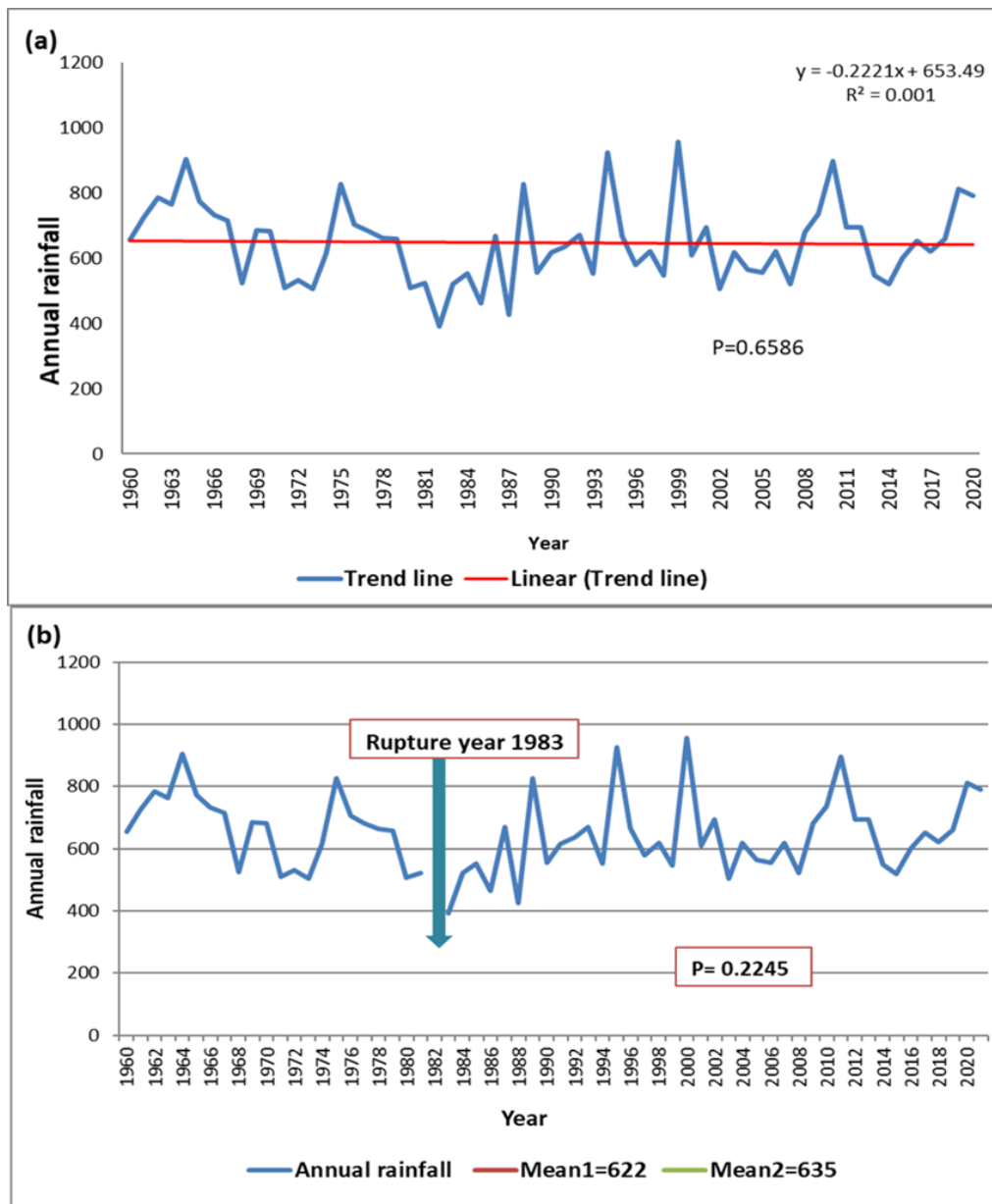
Figure3.5. Trend analysis of annual rainfall (a) and the abrupt change in the trend (b) for Segou
