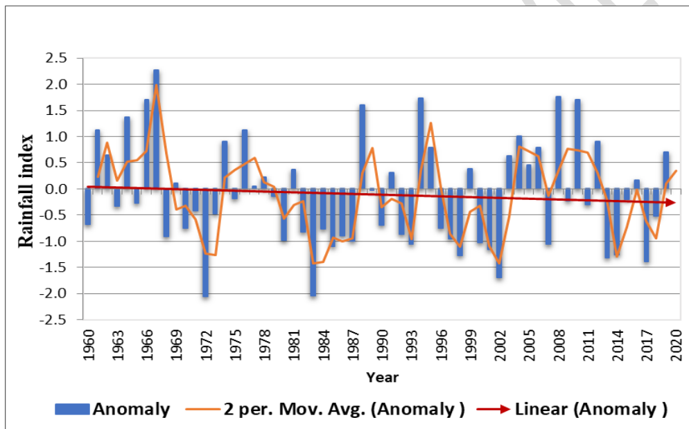
Figure 3.1. Interannual variability of rainfall for Bamako (orange line is moving average and red line is linear trend forecasting)
