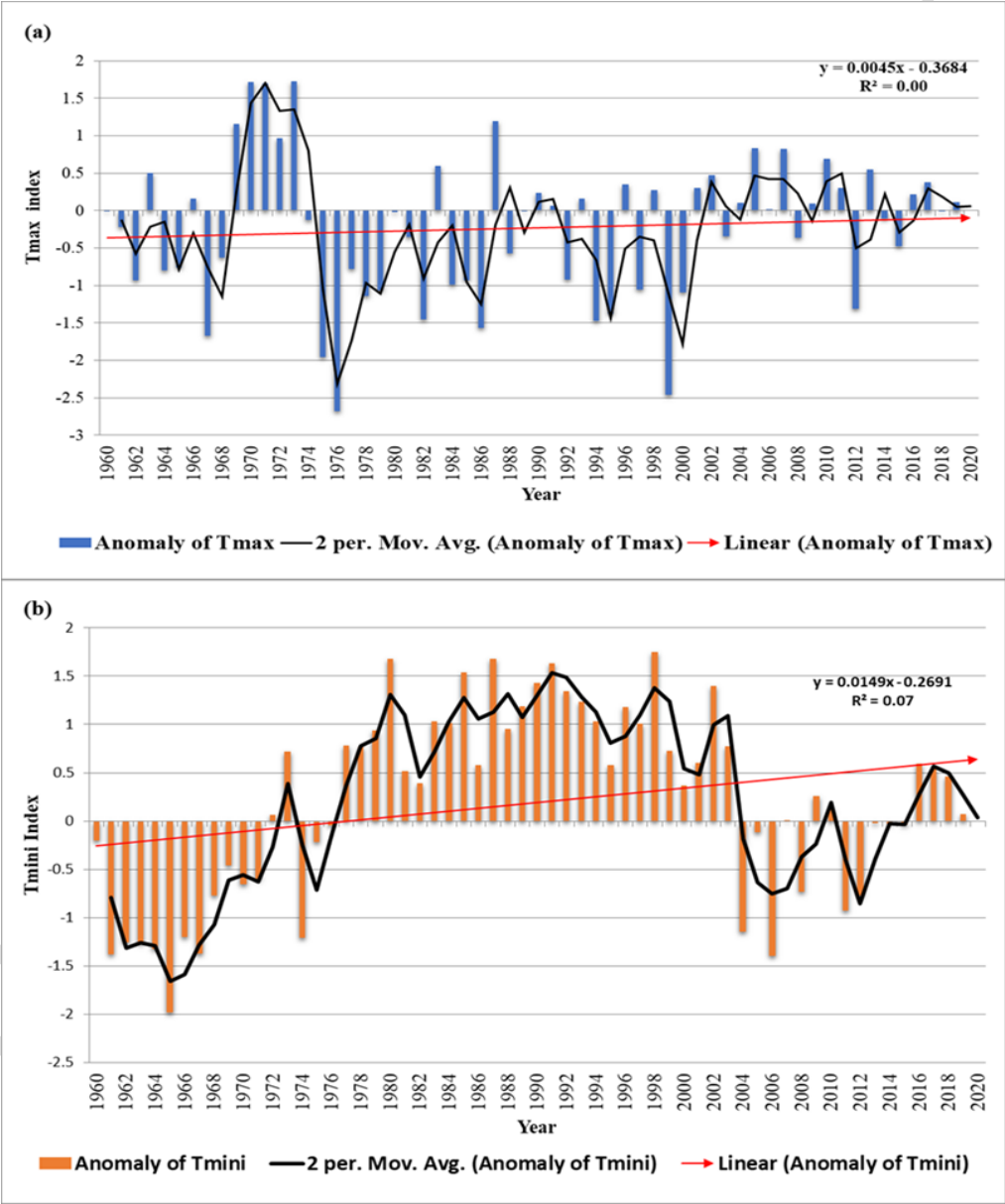
Figure 3.11. Anomaly trend of maximum (a) and minimum temperature (b) for Bamako from 1960-2020 (red line a, b is linear trend and black line is moving average)
