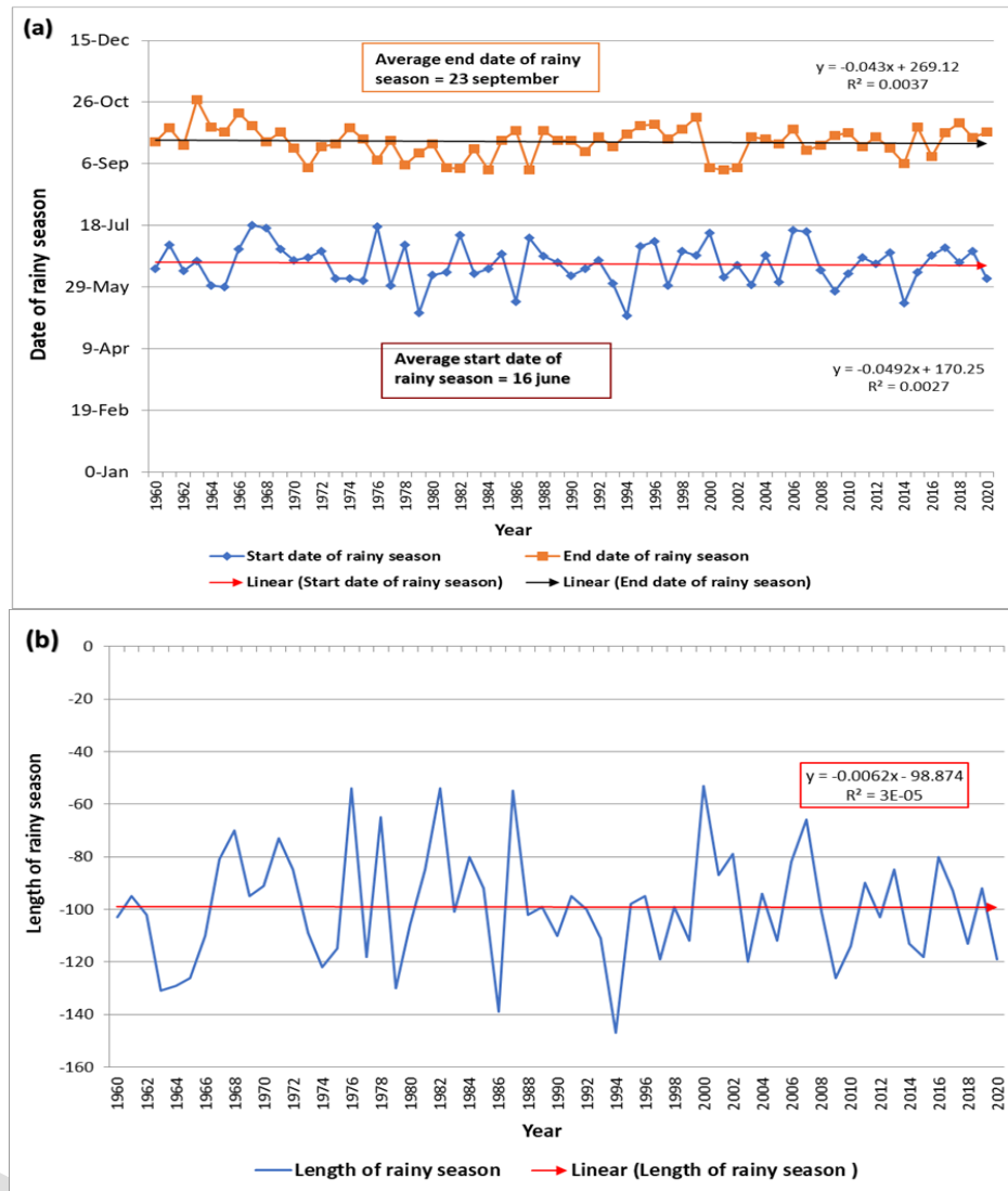
Figure 3.9. Trend of start and end of the rainy season (a), and the length trend of the rainy season (b) for Segou
