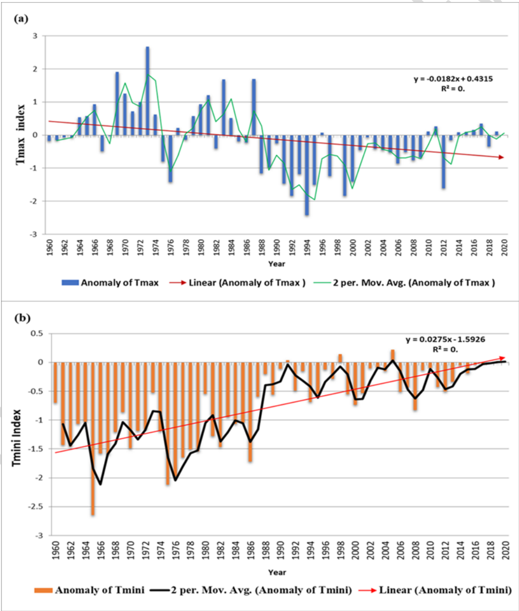
Figure 3.13. Anomaly trend of maximum (a) and minimum temperature (b)for Sikasso from 1960-2020 (red line a, b is linear trend, green and black line is moving average)
