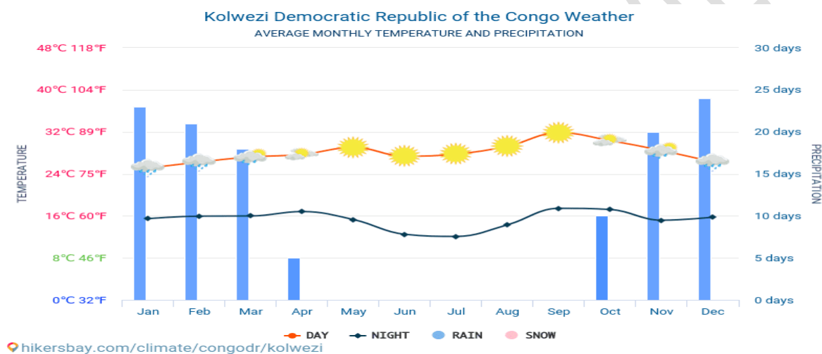
Fig. 1: Distribution of temperature forecasts in Kolwezi in 2023
