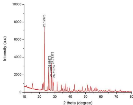
Fig. 4. XRD characterization of nano-S
