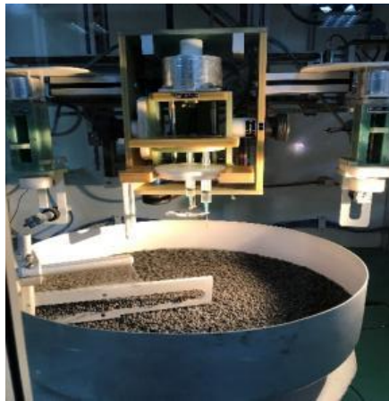
Fig. 2. Vertical electrospinning unit for coating seeds with fibre
