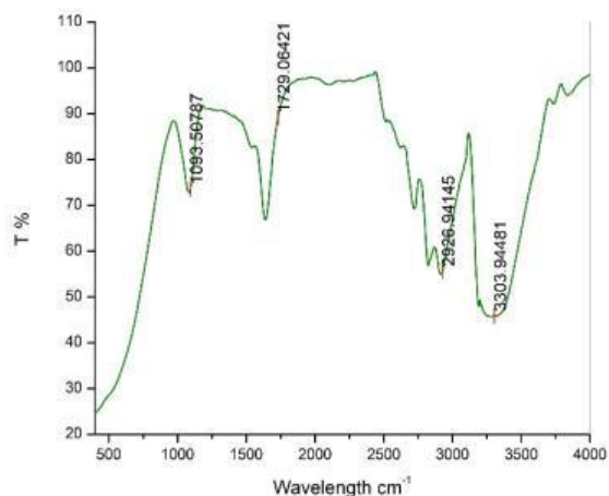
FTIR spectra of PVA nanofiber
