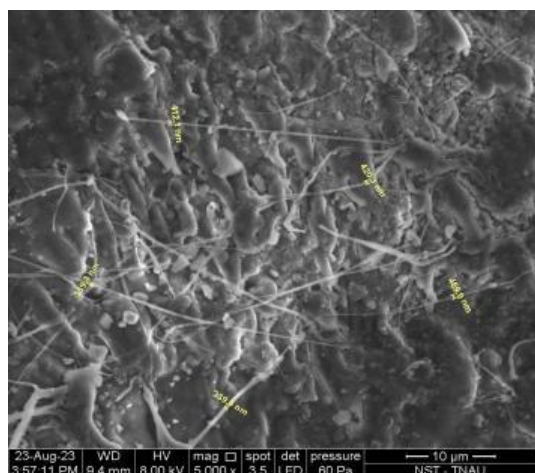
c) SEM image of PVA coated seed
