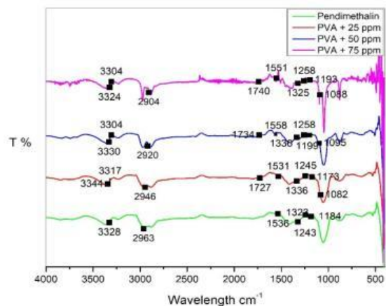
FTIR spectra of PVA nanofiber
