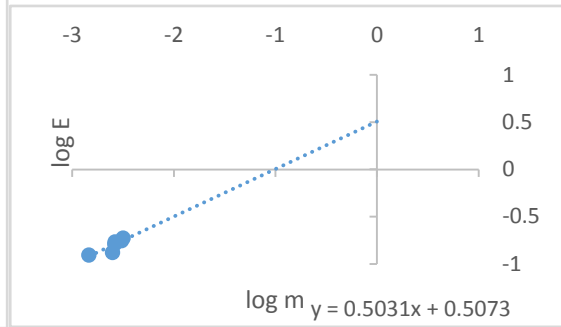
Figure 7: Graph of \log E_{min} against \log m for yam at 66.13 %wb
