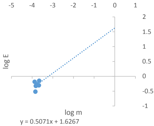
Figure 11: Graph of \log E_{min} against \log m for crayfish at 0.36 %wb
