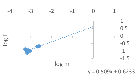
Figure 4: Graph of \log E_{min} against \log m for cassava at 47.64 %wb
