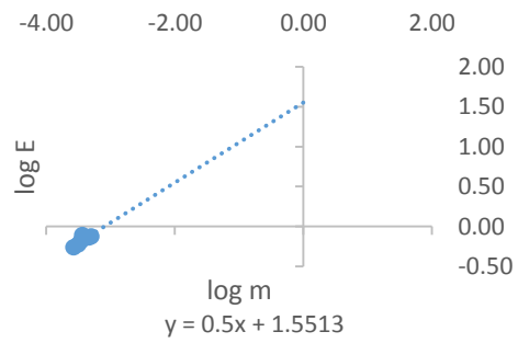
Figure 19: Graph of \log E_{min} against \log m for beans at 2.89 %wb
