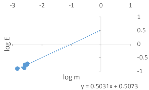
Figure 2: Graph of \log E_{min} against \log m for cassava at 63.14 %wb
