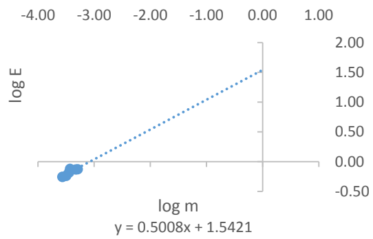
Figure 17: Graph of \log E_{min} against \log m for beans at 4.96 %wb
