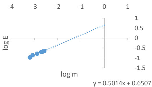
Figure 3: Graph of \log E_{min} against \log m for cassava at 54.54 %wb
