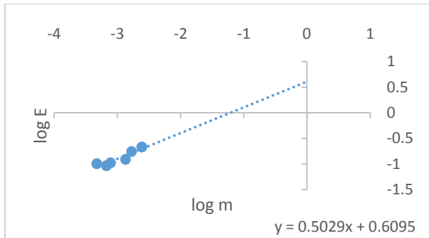
Figure 6: Graph of \log E_{min} against \log m for yam at 47.64 %wb
