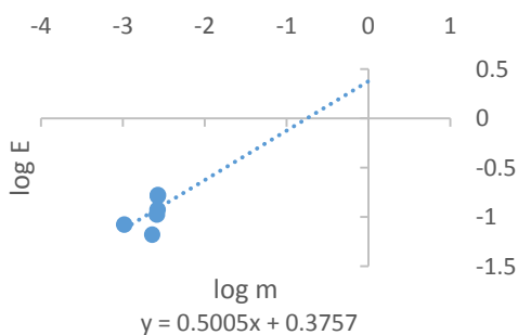
Figure 5: Graph of \log E_{min} against \log m for cassava at 55.00 %wb
