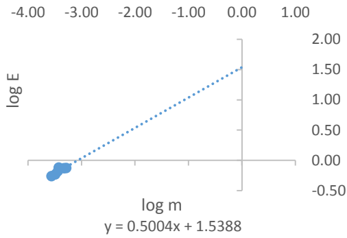
Figure 16: Graph of \log E_{min} against \log m for beans at 5.60 %wb
