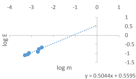
Figure 1: Graph of \log E_{min} against \log m for cassava at 53.83 %wb
