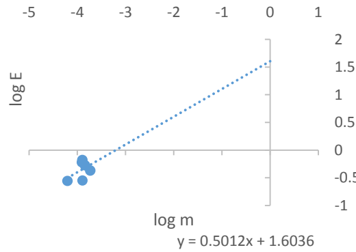
Figure 14: Graph of \log E_{min} against \log m for crayfish at 0.14 %wb
