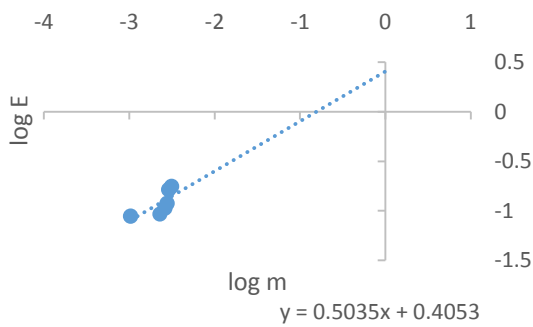
Figure 10: Graph of \log E_{min} against \log m for yam at 54.54 %wb
