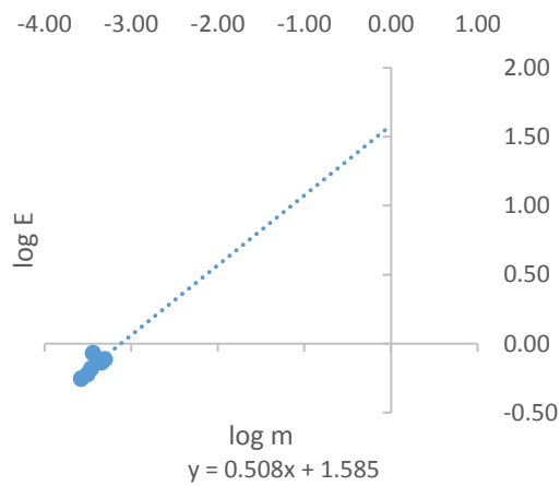
Figure 20: Graph of \log E_{min} against \log m for beans at 1.63 %wb
