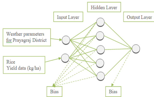
Fig.1. Different layers and different network structural representation of the ANN used in the study.
