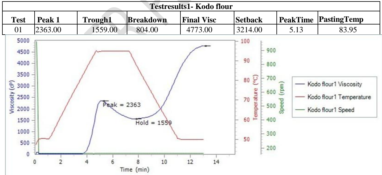
Fig. - 1: Viscosity profile of kodo flour.
