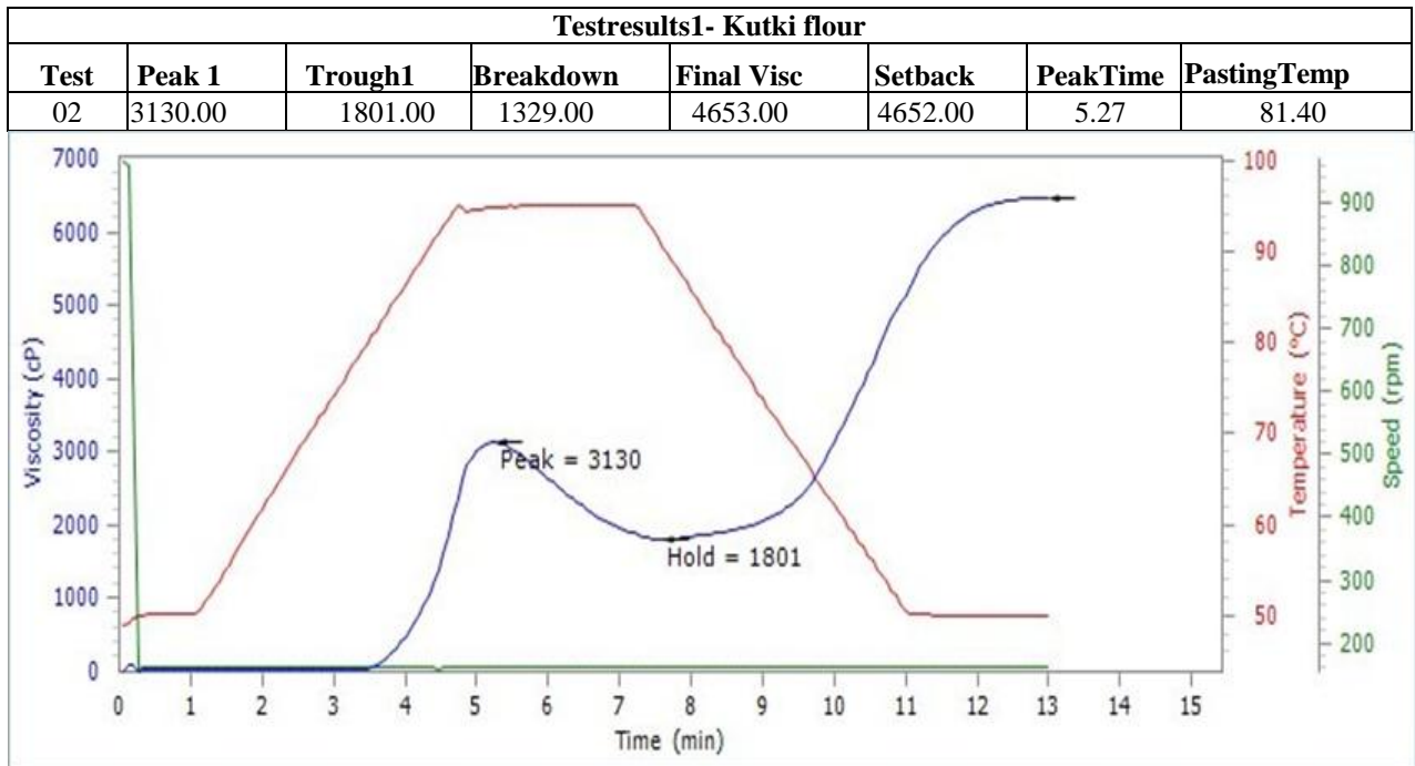
Fig. - 2: Viscosity profile of kutki flour.
