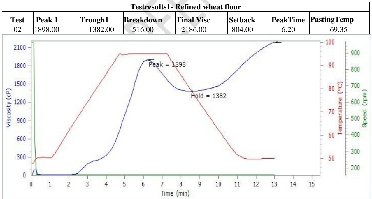
Fig. - 3: Viscosity profile of refined wheat flour.
