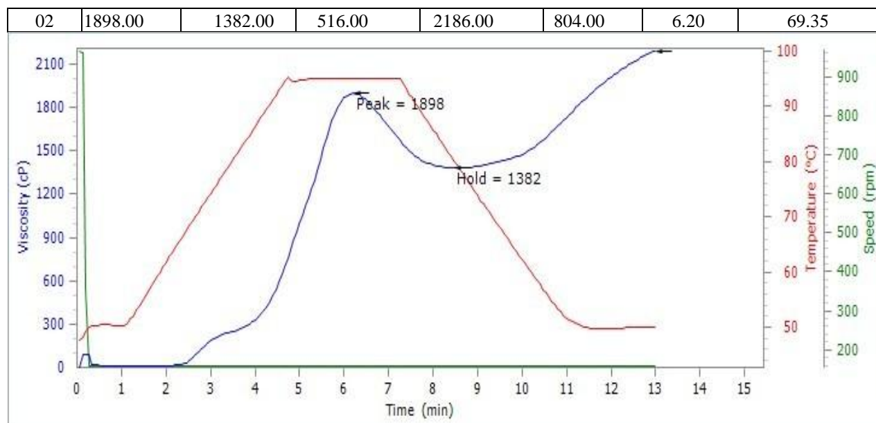
Fig. - 3: Viscosity profile of refined wheat flour.
