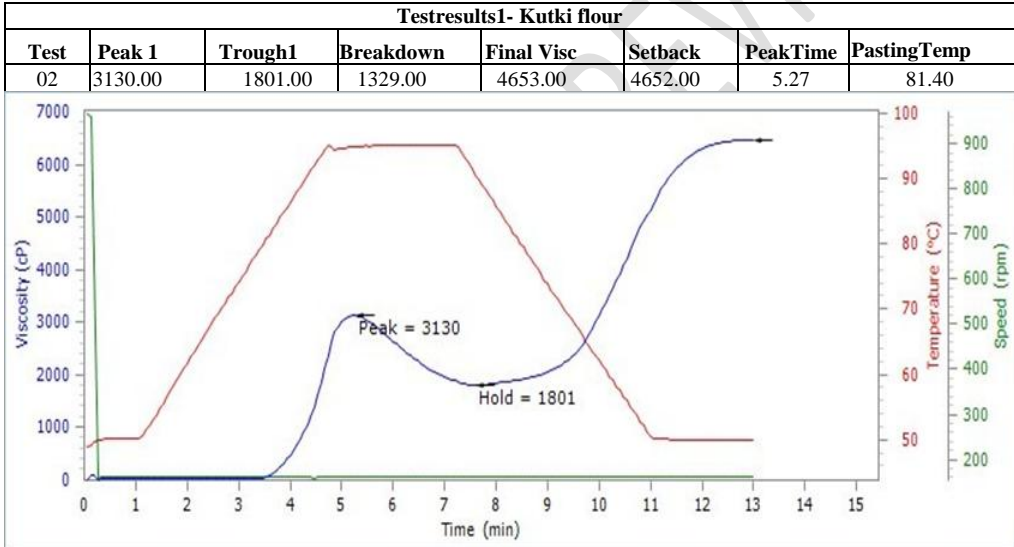
Fig. - 2: Viscosity profile of kutki flour.
