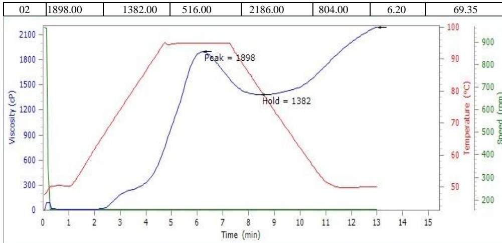
Fig. - 3: Viscosity profile of refined wheat flour.
