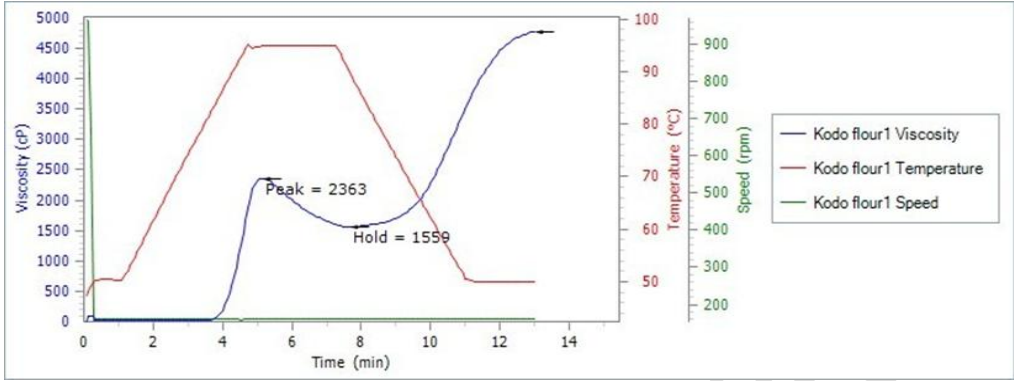
Fig. - 1: Viscosity profile of kodo flour.
