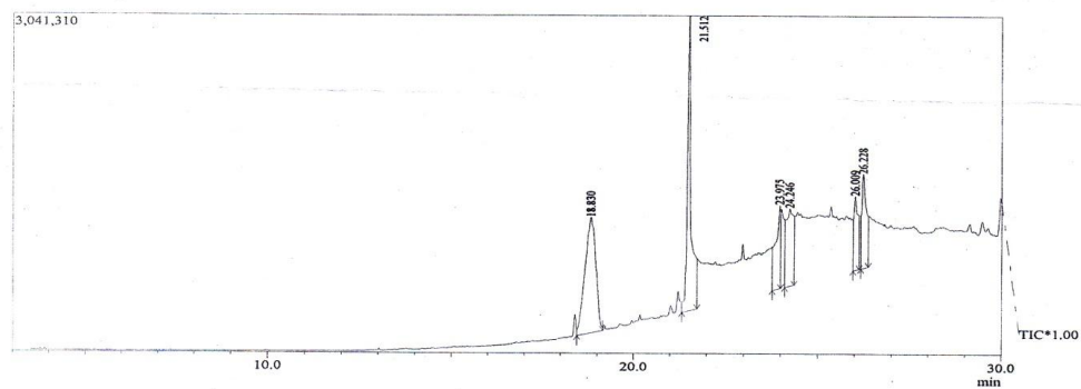
Fig 1: Chromatogram of Mugil parsia Fish oil
