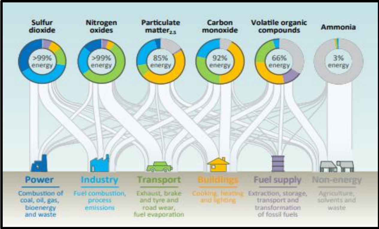
Fig.7. Selected primary air pollutants and their sources (OECD, I. (2016).
