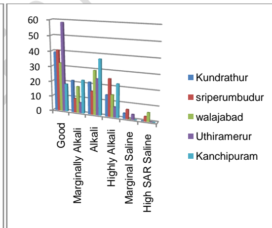
Fig 3. Percentage distribution of groundwater quality in various blocks of Kanchipuram district
