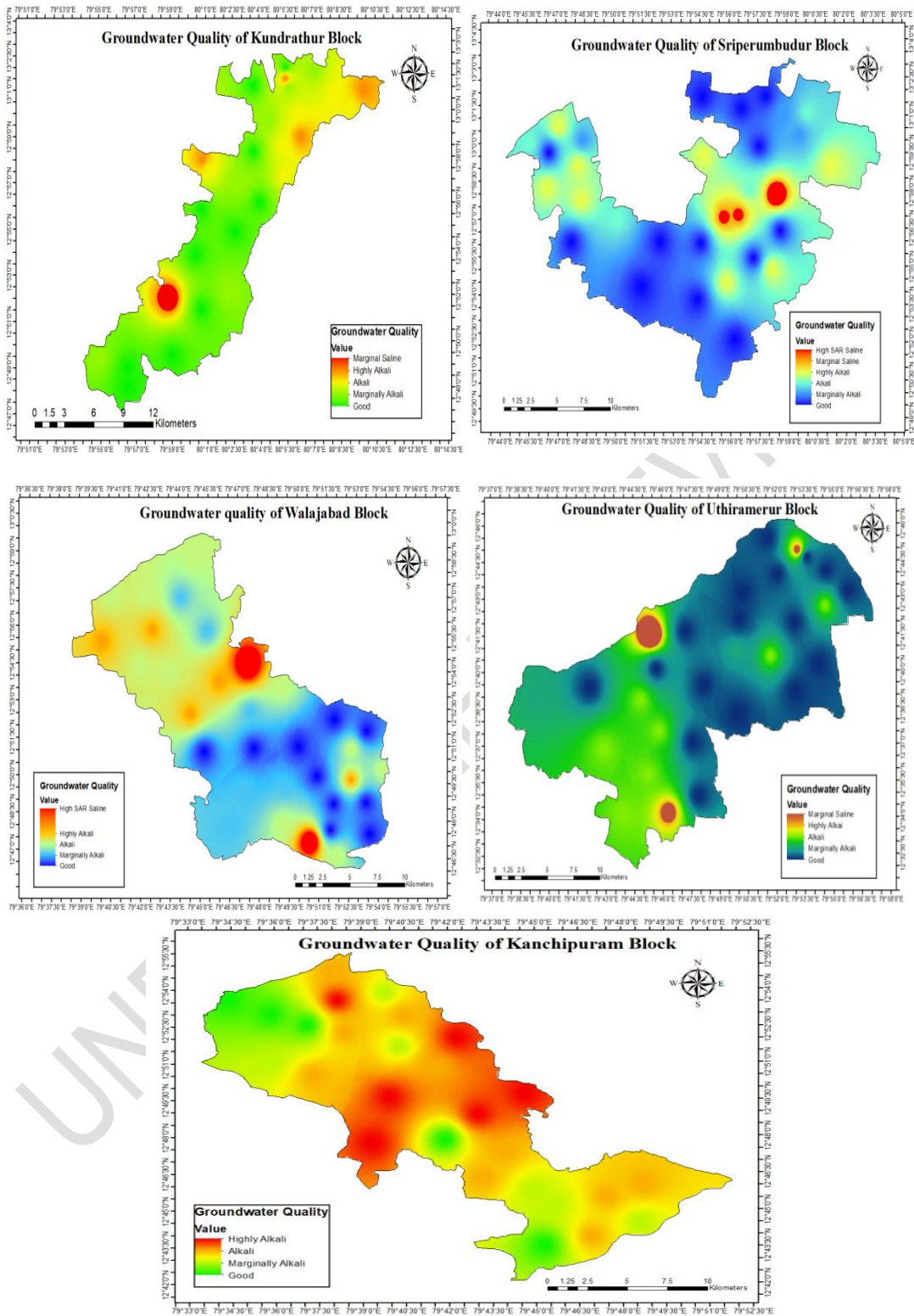
Fig 4. Spatial Distribution for different quality parameters of Groundwater in various blocks of Kanchipuram District
