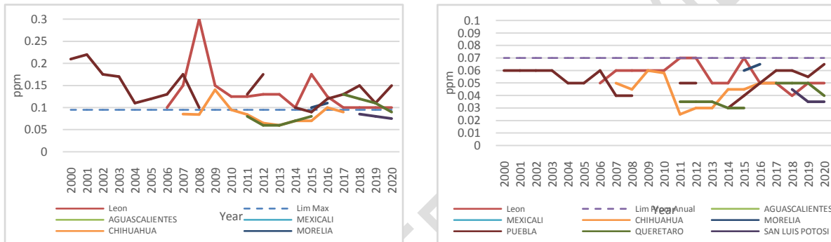
Fig.6 a) Maximum values of O 3 in medium Mexican cities b Annual maximum values of O 3 in medium Mexican cities
