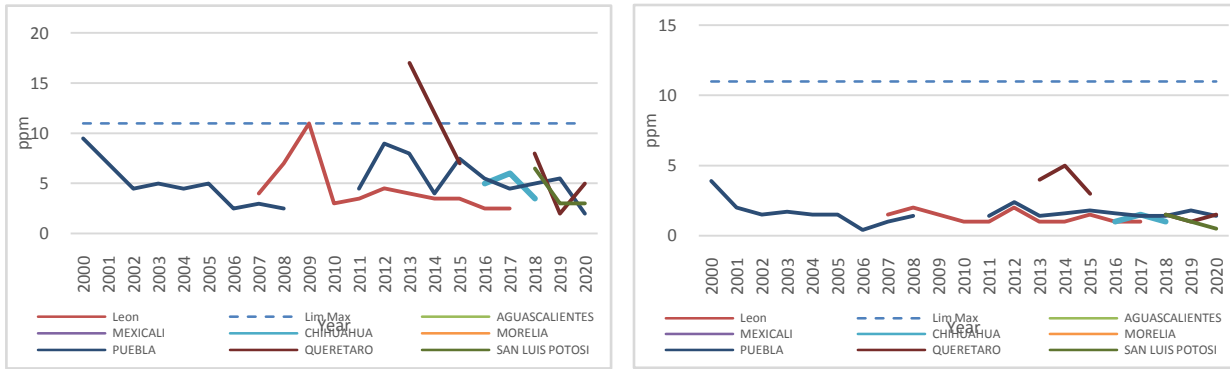
Fig.8 a) Maximum CO values in medium-sized Mexican cities b Annual maximum CO values in medium-sized Mexican cities.
