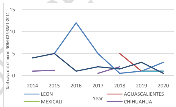
Fig. 5 Percentage of days out of standard NOM-025-SSA1-2014 for \text{PM}_{2.5}
