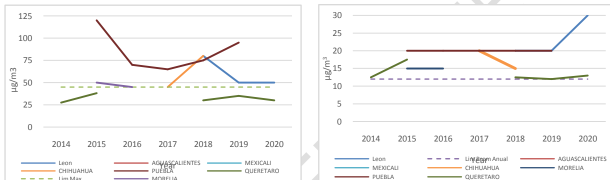
Fig.4 a) Maximum values of \text{PM}_{2.5} in medium Mexican cities b) Annual maximum values of \text{PM}_{2.5} in medium Mexican cities.
