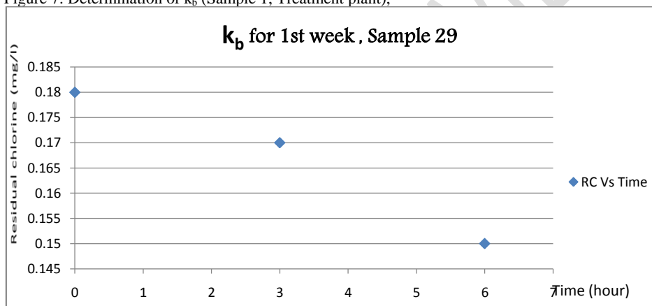
Figure 8: Determination of k_b (Sample 29, Alkammawa),
