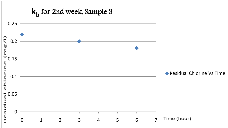
Figure 9: Determination of k_b (Sample 3, Bi-water),
