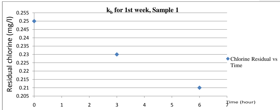
Figure 7: Determination of k_b (Sample 1, Treatment plant),
