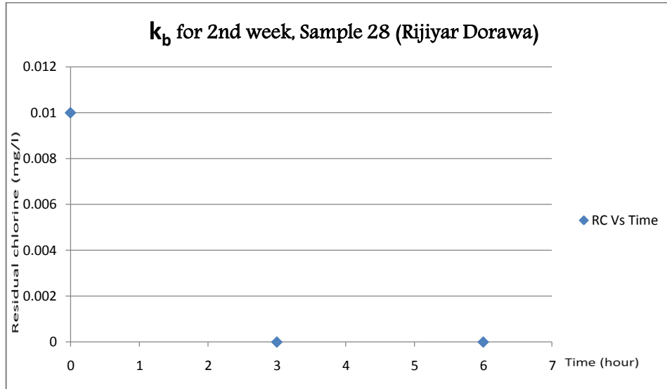
Figure 11: Determination of k_b (Sample 28, RijiyarDorawa),
