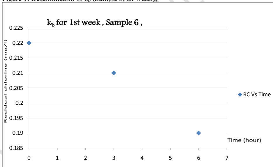
Figure 10: Determination of k_b (Sample 6, Illela garage),
