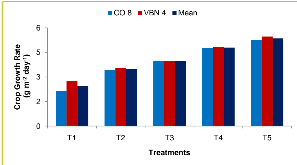
Figure 2. Effect of nutrients and plant growth regulators on Crop Growth Rate of greengram
