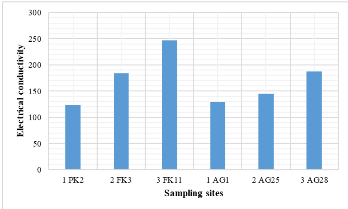
Fig. 6. Soil conductivity ( \mu S/cm ) at sampling sites
