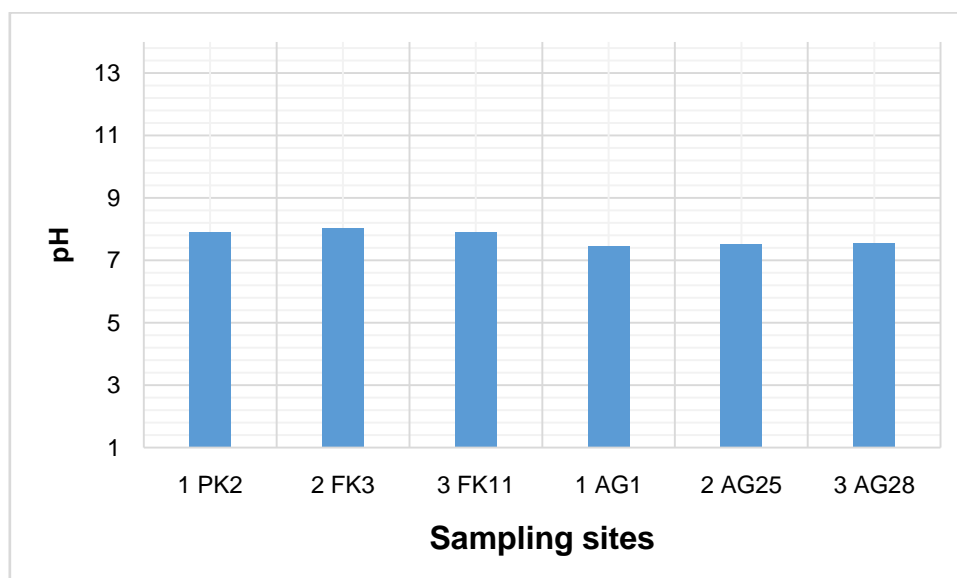
Fig. 7. pH values of sampling sites
