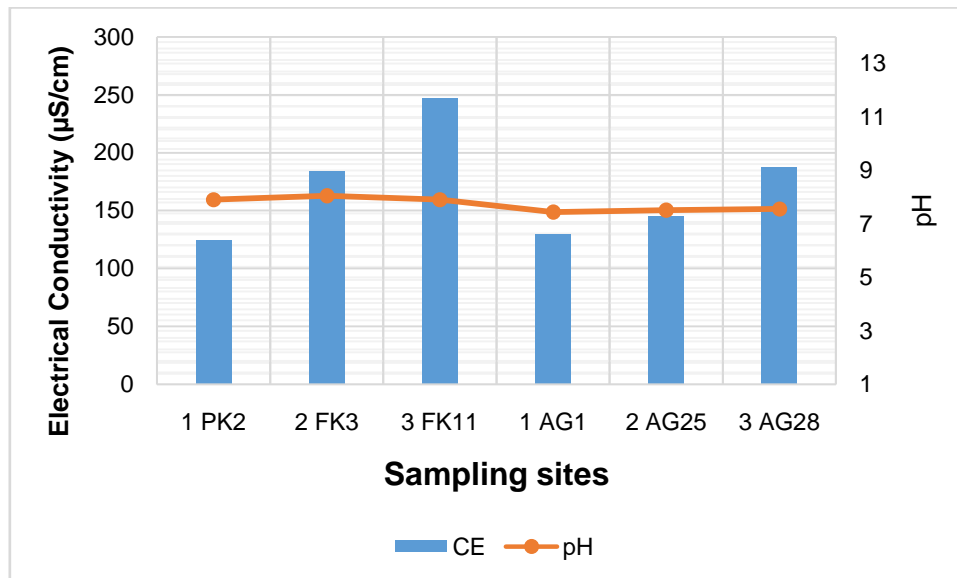
Fig. 8. Electrical conductivity ( \mu\text{S}/\text{cm} ) and soil pH as a function of sampling sites
