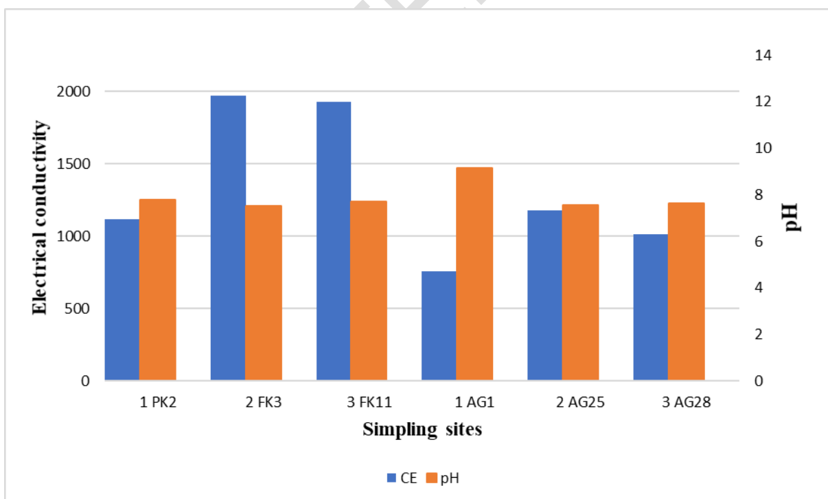
Fig. 5. Values of electrical conductivity ( \mu\text{S}/\text{cm} ) and pH according to sampling sites
