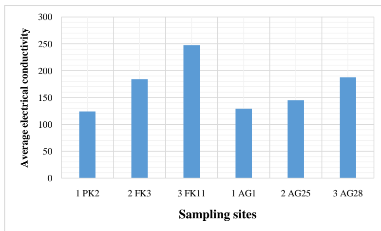
Figure 6 : Average soil conductivity at sampling sites
