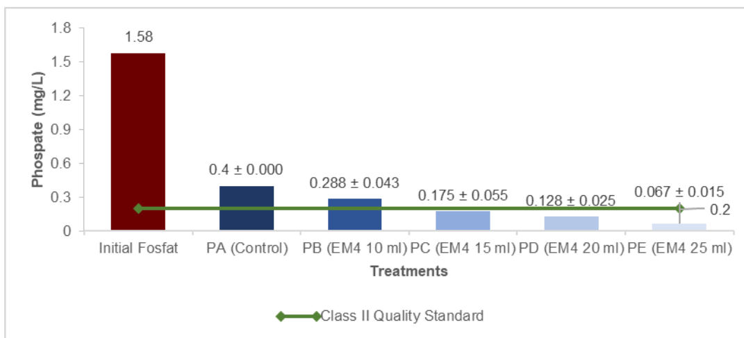
Fig. 4 Phosphate Value
