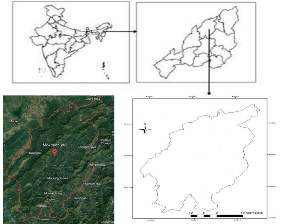
Fig.1. Study sites of jhum cycle in Mokokchung district of Nagaland, Northeast India.
