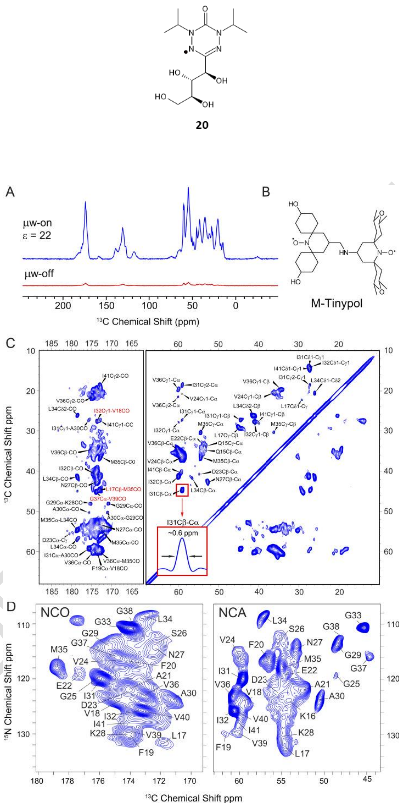
Fig. 7. (A) DNP-enhanced ^{13}\text{C} spectra of 1,3- ^{13}\text{C}_2 /2- ^{13}\text{C} / ^{15}\text{N} -labelled M0A \beta 1-42 illustrating an enhancement of \epsilon = 22 using (B) bis-nitroxide polarising agent M-TinyPol ( 19 ). (C) DNP-enhanced ^{13}\text{C} - ^{13}\text{C} CORD-RFDR spectra of 1,3- ^{13}\text{C}_2 /2- ^{13}\text{C} / ^{15}\text{N} -labelled M0A \beta 1-42. The resolution in the spectrum is comparable to that obtained at ambient temperatures, \sim 0.6 ppm as indicated for I31C \beta -C \alpha . In red are shown the long-range contacts that correspond to the intramolecular monomer
