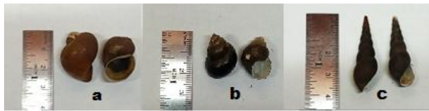
Fig8. Most common macrozoobenthos
