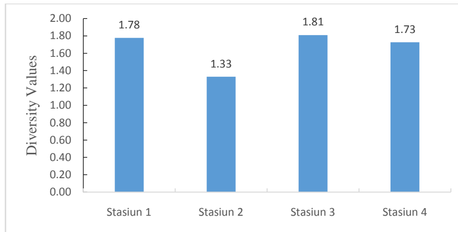
Fig10. Macrozoobenthic diversity values
