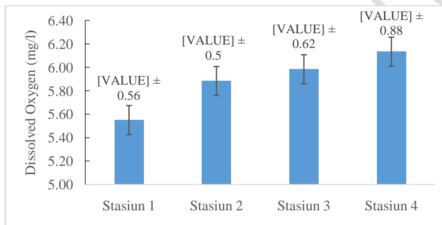
Fig5. Value Dissolved Oxygen (DO)
