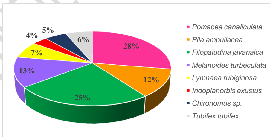
Fig7.The average percentage of each macrozoobenthic species
